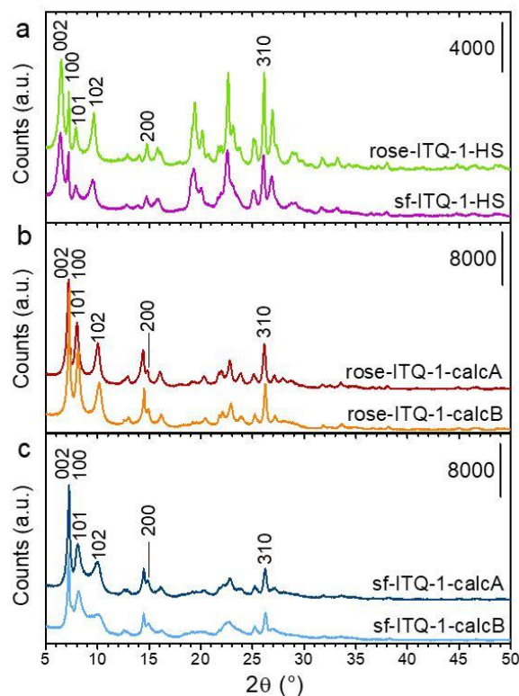
Figure 1. XRD patterns of the as-synthesized rose-ITQ-1-HS and sf-ITQ-1-HS samples (a), calcined rose-ITQ-1-calcA and rose-ITQ-1-calcB (b), and calcined sf-ITQ-1-calcA and sf-ITQ-1-calcB (c) samples.
