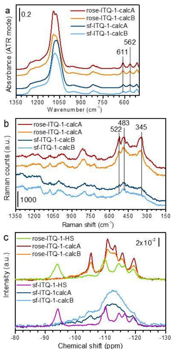
Figure 4. ATR-IR spectra in the 1350-500 \text{cm}^{-1} range (a) and Raman spectra in the 1350-150 \text{cm}^{-1} range (b) of the calcined rose-ITQ-1-calcA, rose-ITQ-1-calcB, sf-ITQ-1-calcA, sf-ITQ-1-calcB samples, and ^{29}\text{Si} -OP-NMR spectra of the as-synthesized rose-ITQ-1-HS and sf-ITQ-1-HS and calcined rose-ITQ-1-calcA, rose-ITQ-1-calcB, sf-ITQ-1-calcA and sf-ITQ-1-calcB samples (c).
