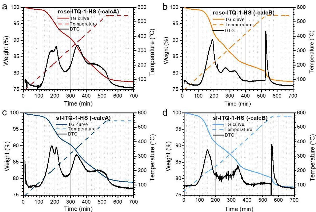
Figure 6. TG analyses of rose-ITQ-1-HS sample calcined with procedure A (a), rose-ITQ-1-HS sample calcined with procedure B (b), sf-ITQ-1-HS sample calcined with procedure A (c) and sf-ITQ-1-HS sample calcined with procedure B (d). Procedure A : 1 °C/min up to 550 °C under dry air, followed by 3 h in isothermal conditions under the same flux. Procedure B : 1 °C/min up to 580 °C under N 2 flux, followed by 3 h in isothermal conditions under dry air.
