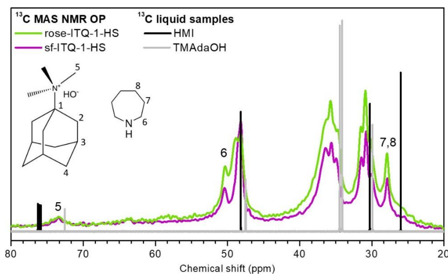
Figure 5. 13 C OP-NMR spectra of as-synthesized rose-ITQ-1-HS and sf-ITQ-1-HS samples, compared with the liquid phase spectra of the pure OSDAs (HMI and TMAdaOH).
