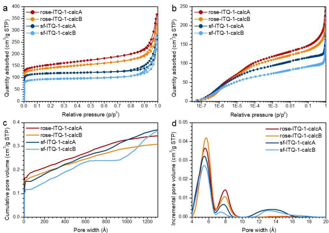
Figure 3. Volumetric N 2 adsorption/desorption isotherms at - 196 °C in the whole relative pressure range, plotted in linear (a) and semi-logarithmic scale (b). Cumulative pore volume plot in the 0 – 1300 Å pore size range (c) and pore size distributions in the micropore size range (< 20 Å, points connected by a B-spline function) (d), computed by NL-DFT method applied to the N 2 adsorption isotherms in the whole relative pressure range.
