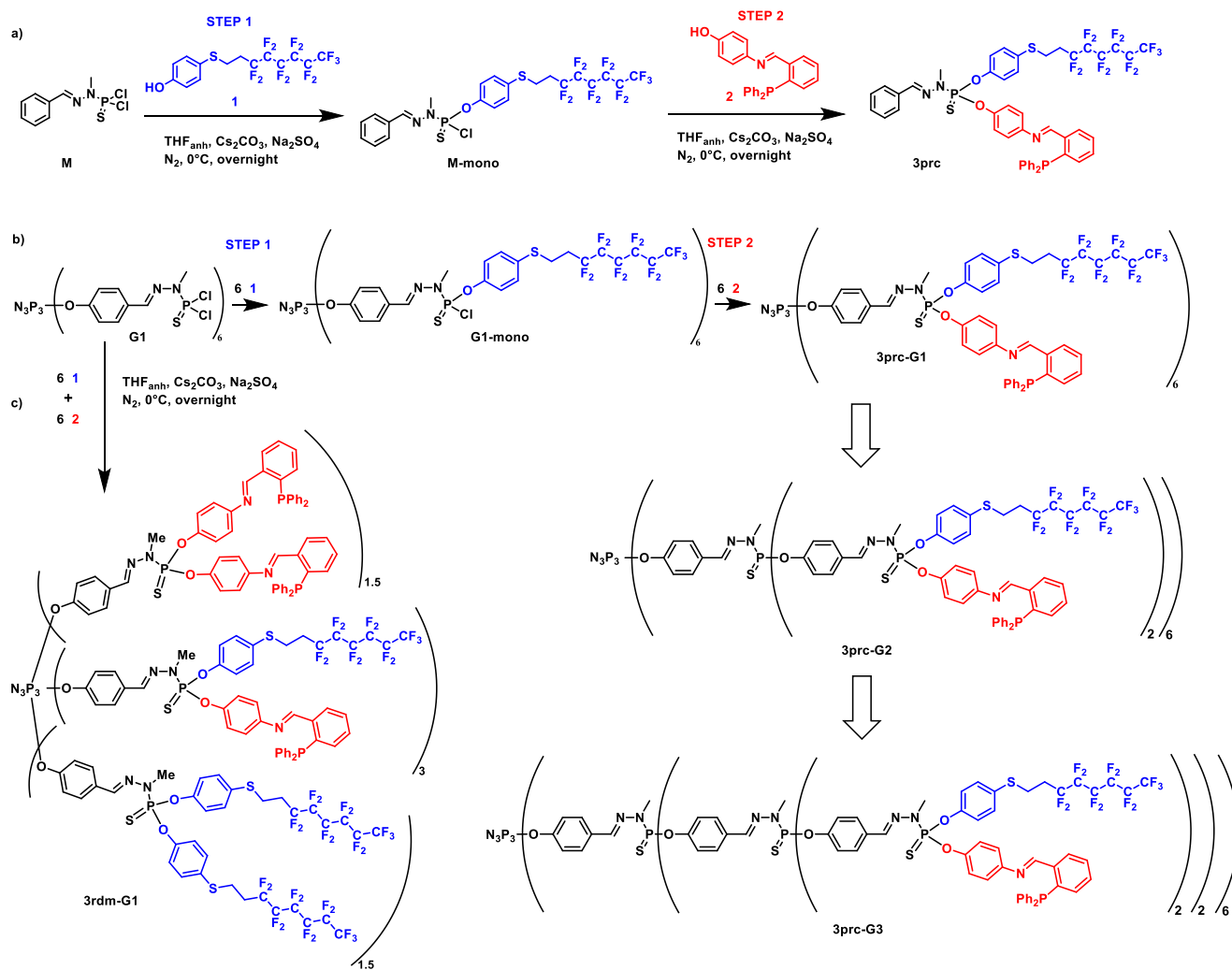
Scheme 1. Synthesis of the (a) Precisely Difunctionalized Monomer (3prc) (b) of the First-Generation Dendrimer (3prc-G1 Reaction Also Carried out to Synthesize 3prc-G2 and 3prc-G3) (c) and of 3rdm-G1 (Reaction Also Carried out to Synthesize 3rdm-G2 and 3rdm-G3); Structure of 3prc-G2 and 3prc-G3
