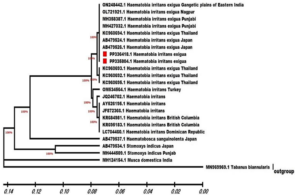
Fig. 10. Unweighted Pair Group Method with Arithmetic Mean (UPGMA) Tree of COI gene
