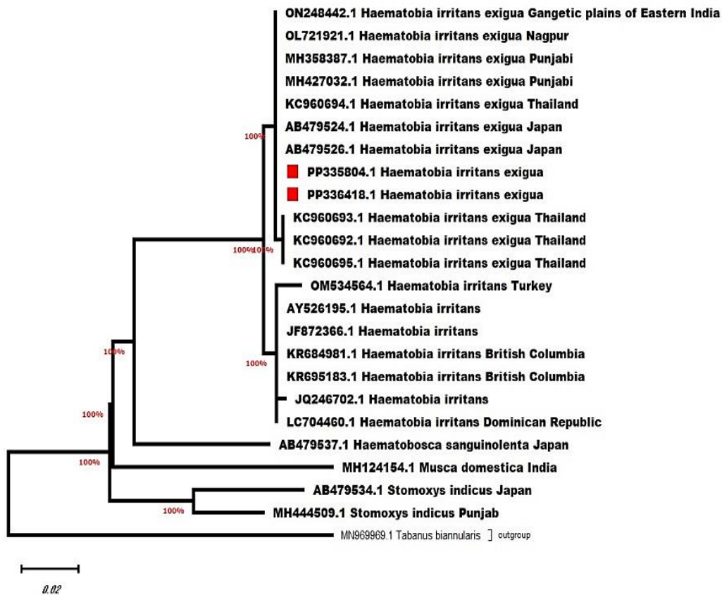
Fig. 9. Neighbour-Joining Tree of COI gene
