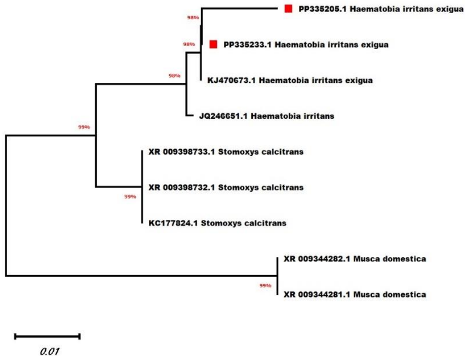
Fig. 10. Unweighted Pair Group Method with Arithmetic Mean (UPGMA) Tree of COI gene
