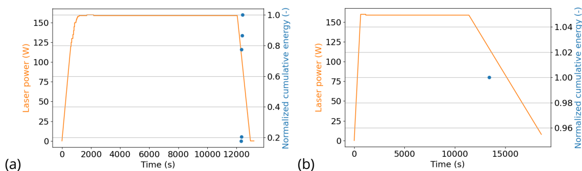
Figure 18: Acoustic emission during the first thermomechanical loading cycle, for (a) 15 min and (b) 2 h cooling.
