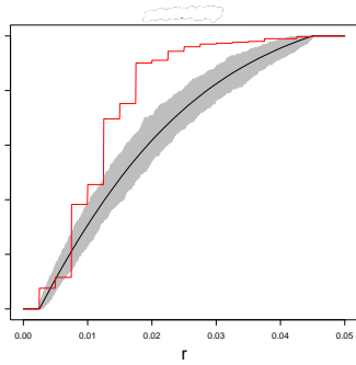
(a) Strauss point process
