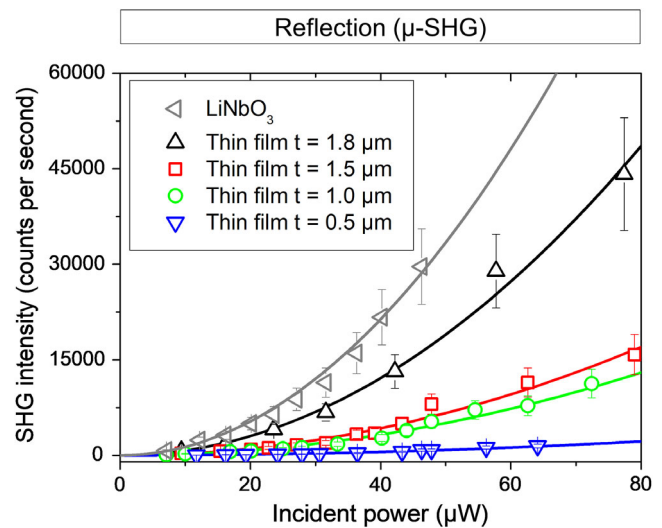
Figure 8. In the structured zone, SHG intensity as a function of the incident power for the films of different thicknesses measured by specular reflection SHG microscopy (with a linear polarization) as well as for the lithium niobate single crystal (in gray) used as a reference. The films are oriented so that the linear polarization is perpendicular to the imprinted line and the lithium niobate crystal is oriented so that its c -axis is collinear to the linear polarization and so that \chi_{zzz}^{(2)} is probed. The continuous lines correspond to quadratic fits. Note that the fitting coefficient corresponding to lithium niobate is 13.36.
