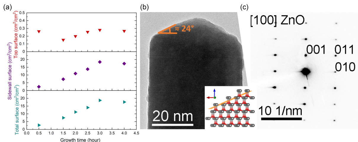
Figure 4. a) Evolution of the top surface area, sidewall surface area, and total surface area of ZnO NWs grown by CBD as a function of growth time, as determined over a substrate surface area of one \text{cm}^2 . b) HRTEM image of a single ZnO NW grown by CBD for a growth time of 3 h. The inset is a schematic of the wurtzite structure of ZnO along the Zn-polar c -axis cut parallel to the semipolar (10\bar{1}4) plane. c) Corresponding SAED pattern showing its orientation along the polar c -axis.
