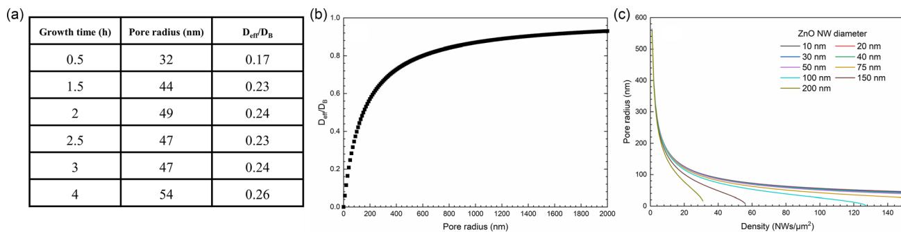
Figure 6. a) Pore radius and D_{\text{eff}}/D_B ratio of MO organic dye for different growth times of ZnO NWs by CBD. b) Evolution of the D_{\text{eff}}/D_B ratio as a function of pore radius. c) Evolution of the pore radius as a function of the apparent density of ZnO NWs for different mean diameters.
