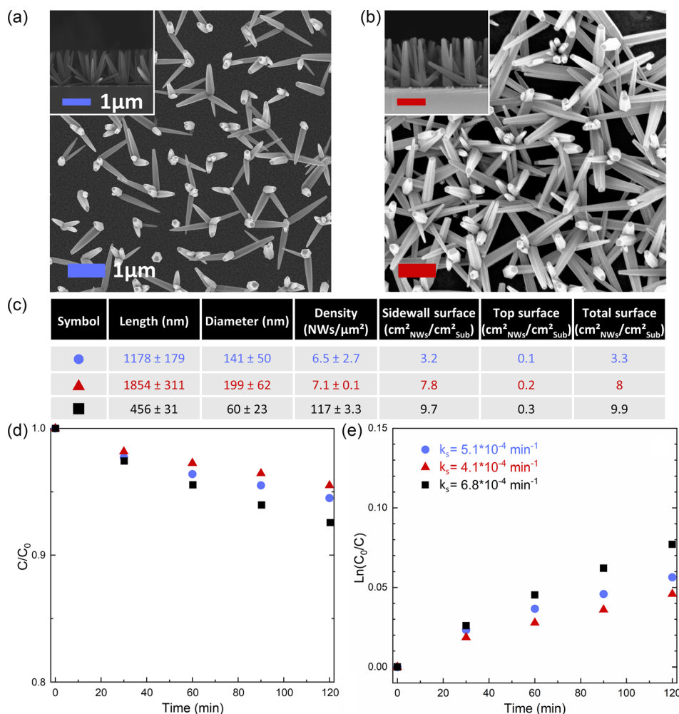
Figure 7. a) Top-view and cross-sectional view FESEM images of ordered ZnO NR arrays grown by CBD for a growth time of 1 h 05 min and b) 1 h 45 min. The scale bar denoting 1 \mu\text{m} is the same for each top-view and cross-sectional view FESEM image, respectively. c) Mean length, diameter, density, sidewall surface area, top surface area, and total surface area of ordered ZnO NRs and spontaneously grown ZnO NWs. d) Evolution of the residual (C) over initial ( C_0 ) concentration ratios of MO organic dye as a function of time for ordered ZnO NR arrays and spontaneously grown ZnO NW arrays. e) Corresponding photocatalytic degradation kinetics plots of MO organic dye. The symbols (●) and (▲) stand for ordered ZnO NR arrays grown for 1 h 05 min and 1 h 45 min, respectively, while the symbol (■) stand for spontaneously grown ZnO NWs for 1 h 45 min.
