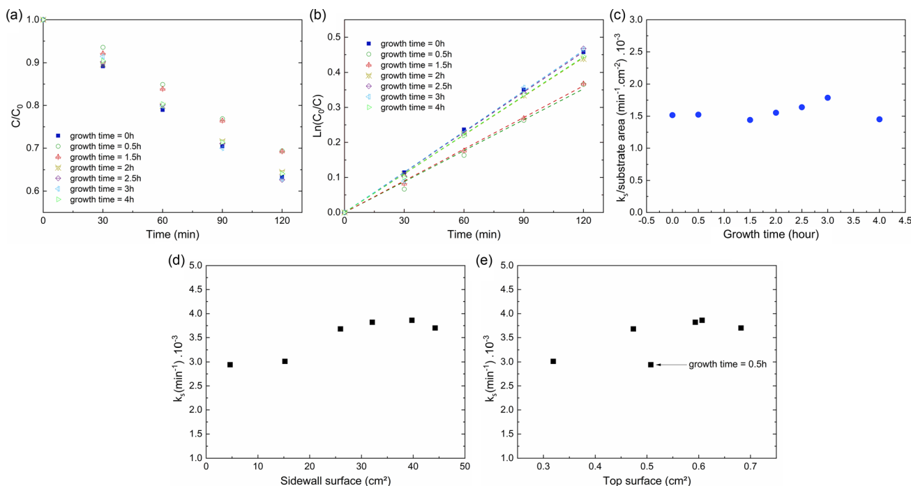
Figure 5. a) Evolution of the residual ( C ) over initial ( C_0 ) concentration ratios of MO organic dye as a function of time for the polycrystalline ZnO seed layer and for ZnO NWs grown by CBD for a growth time ranging from 0.5 to 4 h. b) Corresponding photocatalytic degradation kinetics plots of MO organic dye. The dashed lines represent the linear fit from the Langmuir–Hinshelwood model in Equation (1). Evolutions of the k_S apparent reaction rate constant as a function of the c) growth time, d) sidewall surface area, and e) top surface area of ZnO NWs.
