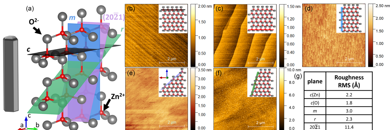
Figure 1. a) Schematic of the wurtzite structure of ZnO along the Zn-polar c -axis, representing the different polar, nonpolar, and semipolar planes considered. AFM maps in tapping mode of ZnO single crystals with the b) Zn-polar (0001) +c -plane, c) O-polar (000 \bar{1} ) -c -plane, d) nonpolar (10 \bar{1} 0) m -plane, e) semipolar (10 \bar{1} 2) r -plane, and f) semipolar (20 \bar{1} ) plane orientations. The insets represent the schematic of the wurtzite structure of ZnO along the Zn-polar c -axis cut parallel to the orientations considered. The small red (resp. large grey) spheres represent the Zn atoms (resp. O atoms). g) RMS roughness of ZnO single crystals with the different orientations.
