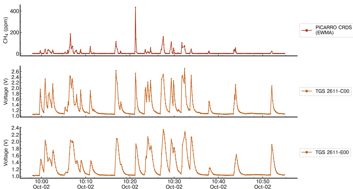
Figure A3. Comparison of the response of the TGS 2611-C00 and TGS 2611-E00 sensors with CH_4 measurements from the reference instrument for release no. 2, which contains spikes with high concentration. The spikes observed on the TGS sensors corresponding to amplitudes from 100 ppm to more than 200 ppm are not distinguishable from spikes with amplitudes lower than 50 ppm.
