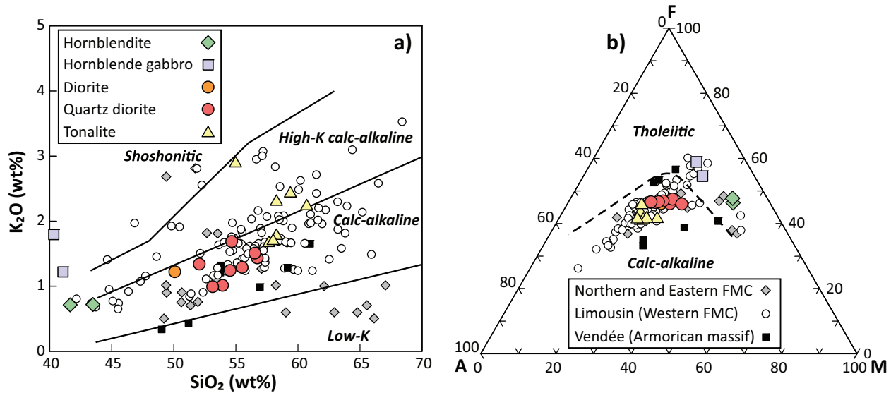
Fig. 5. Classification of Late Devonian – Early Carboniferous calc-alkaline plutonic rocks from the French Massif Central and the Armorican Massif in the K_2O - SiO_2 diagram (a) and the AFM triangle plot (b). Literature data (white, black and grey symbols) are from Pfeiffer (1986); Shaw et al., (1993); Cuney et al., (2001) and Pin and Paquette (2002).
