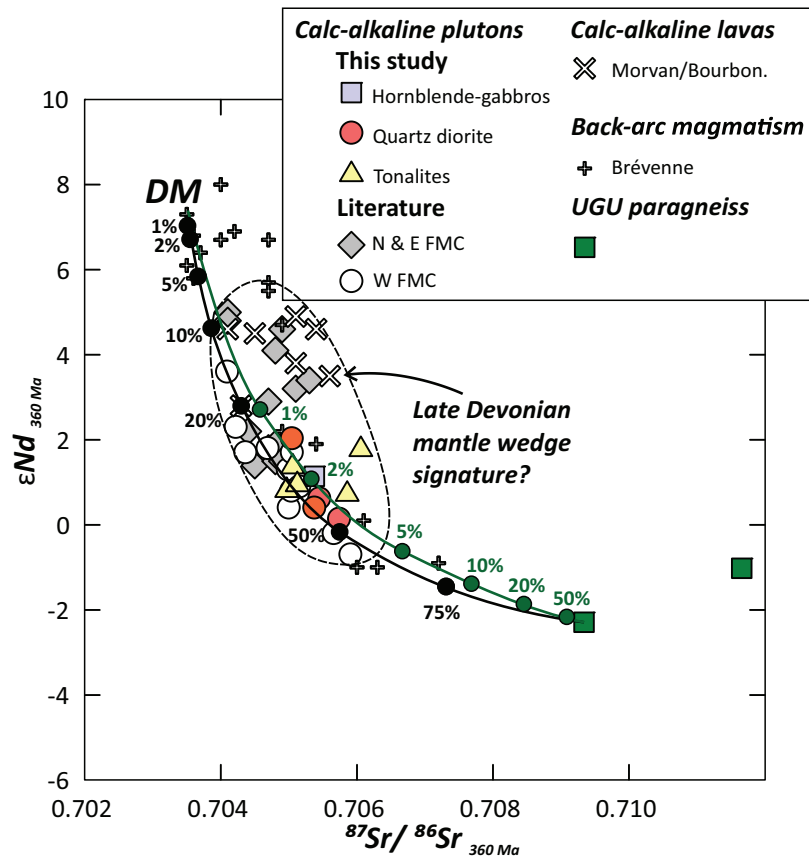
Fig.8. Sr-Nd isotopic diagram for calc-alkaline lavas/plutons from the French Massif Central (this study, Shaw et al. , 1993; Cuney et al. , 2001; Pin and Paquette, 2002) and for Brévenne back-arc magmatism (Pin and Paquette, 1997). Also shown, the composition of the Depleted Mantle (DM) at 360 Ma (calculated with the data of Salters and Stracke, 2004), the probable signature of the mantle wedge around 360 Ma as attested by calc-alkaline magmatism arc like magmatism. The green dotted mixing hyperbola represent mixing between Depleted Mantle and a UGU paragneiss to model mixing of the mantle source with sediments buried by subduction while the black mixing dotted curve simulates contamination of a depleted basalt by a UGU paragneiss to reproduce continental assimilation. Values in % indicate the relative mass of sedimentary component in the mix.
