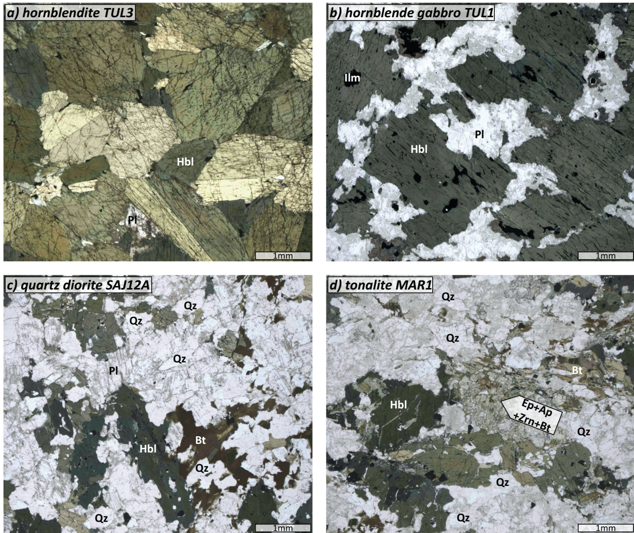
Fig.3. Representative microphotographs of hornblendite TUL3 (a), hornblende gabbro TUL1 (b), hornblende-biotite quartz diorite SAJ12A (c) and hornblende-biotite tonalite MAR1 (d). Despite post-magmatic alteration, igneous textures are generally preserved (a, b, c) but a weak foliation can develop locally (d). Note the interstitial epidote-apatite-zircon-biotite cluster in sample MAR1 (d).
