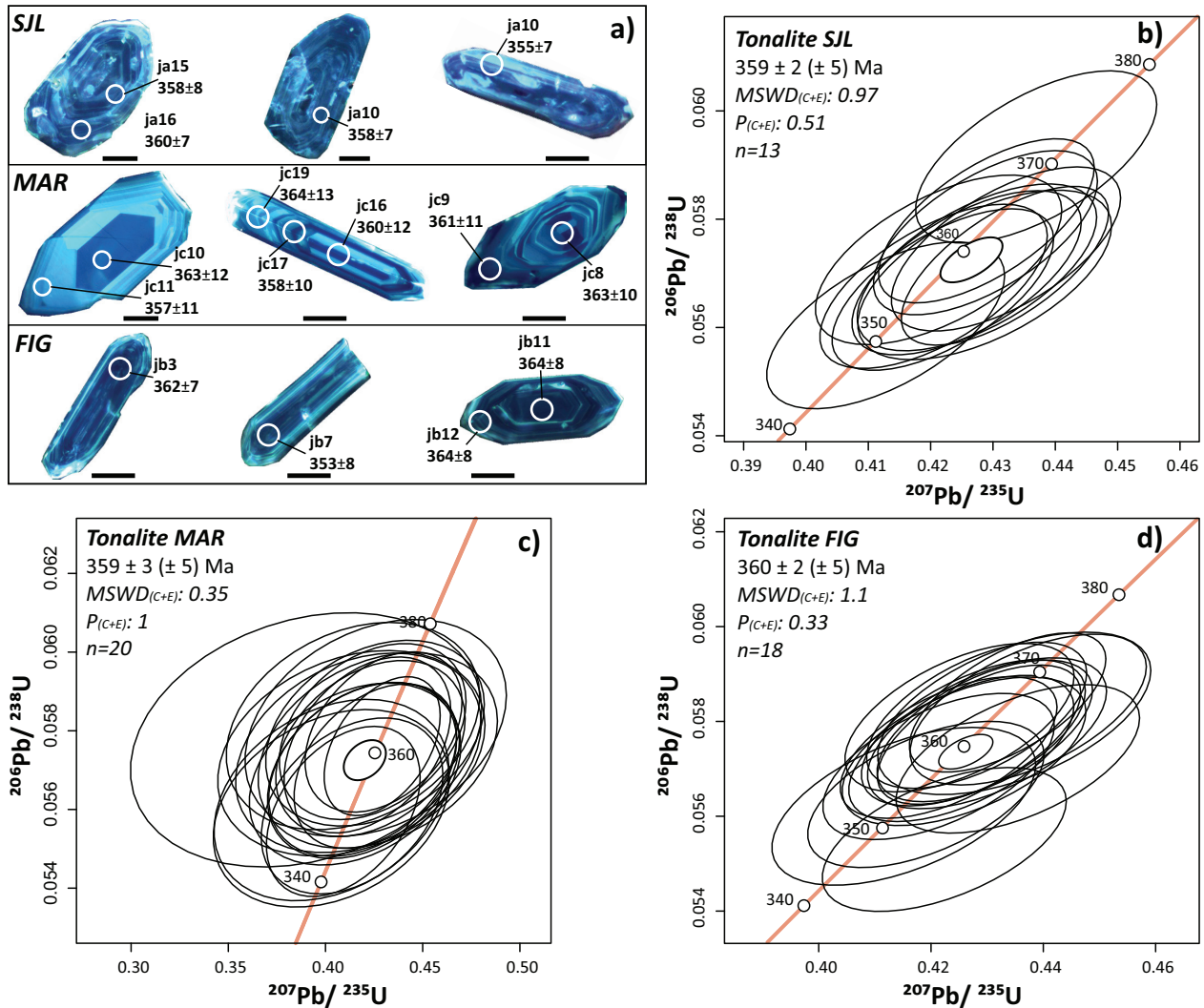
Fig.9. Results of in situ LA-ICP-MS U-Pb zircon dating. (a) Cathodoluminescence images of representative zircon grains. Scale bars represent a length of 20 \mu\text{m} and the quoted ages in Ma are calculated from ^{206}\text{Pb}/^{238}\text{U} ratios. (b, c, d) Concordia plots for tonalites SJL, MAR and FIG, respectively. MSWD and p -value are for concordance and equivalence. The two uncertainties are reported as 2\sigma .
