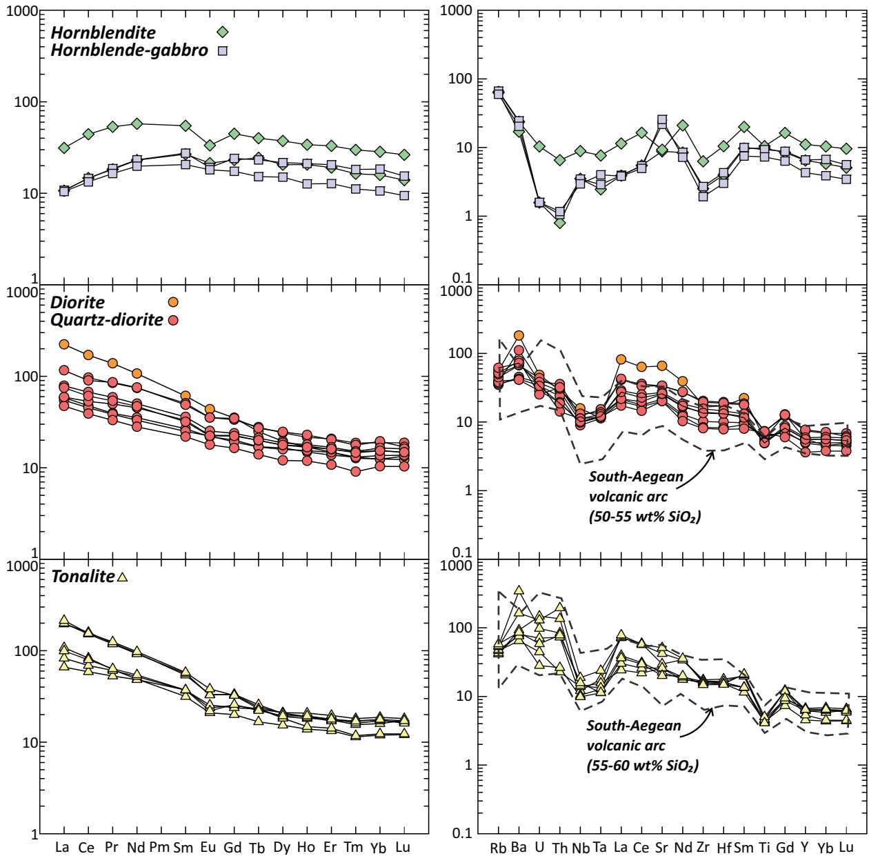
Fig. 7. Chondrite-normalized REE patterns and primitive mantle normalized multi-element diagrams for the calc-alkaline plutonic rocks investigated in this study. The compositions of volcanic rocks from the South Aegean arc are extracted from the Georoc database. Normalization values are from McDonough and Sun (1995).
