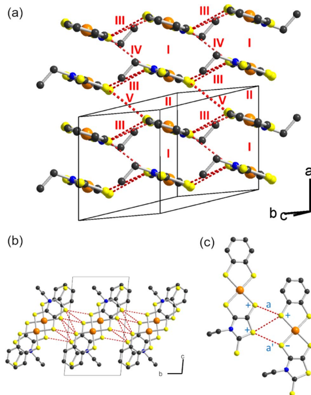
Fig. 7 (a) Layers of the crystal structure of the radical 1' where the different intermolecular interactions are noted. The S...S contacts shorter than 3.8 Å are shown as dotted red lines. (b) Top view of the layer. (c) Intermolecular interaction III: the + and - signs refer to the sign of the S p z orbital in the SOMO showing that interactions a and a' almost cancel.
