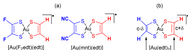
Scheme 4 Model complexes theoretically investigated with (a) [Au(R,Redt)(edt)]* (R=F, CN) complexes, (b) [Au(edt) 2 ]* complexes with constrained C=C bonds.
