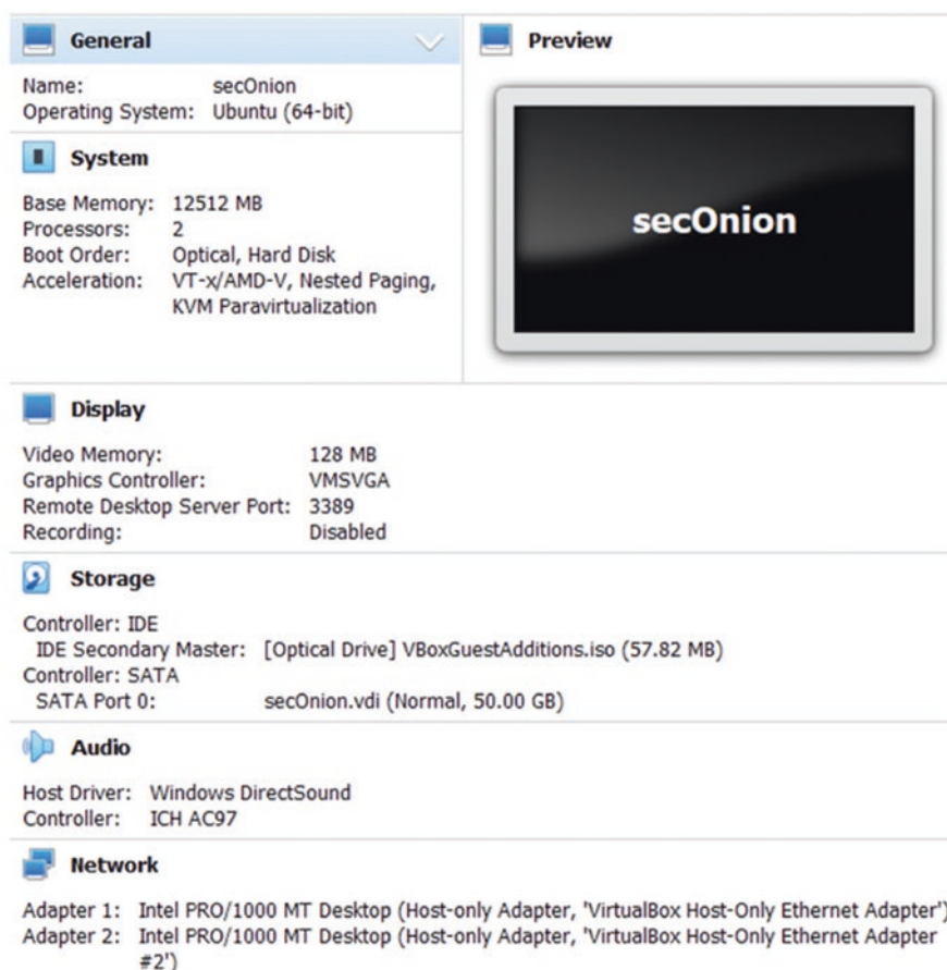
Fig. 7.3 Security Onion VM specifications
