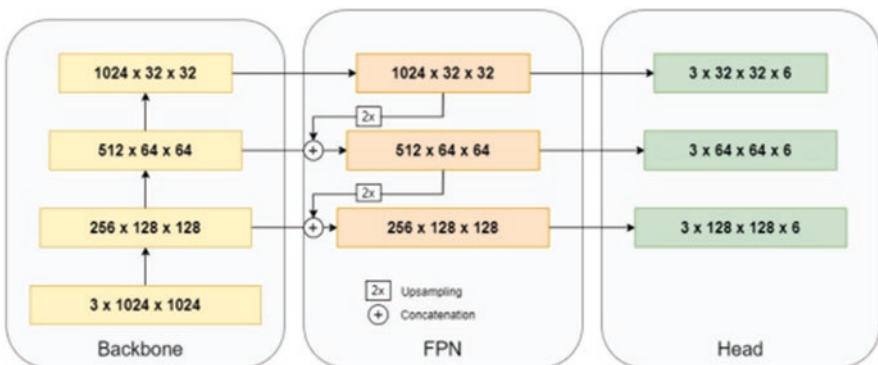
Fig. 5.12 An illustration of multiple convolutional layers and multidimensional matrices, such as the feature maps with 1024 \times 1024 input resolution (Tsiktisiris et al., 2022)
