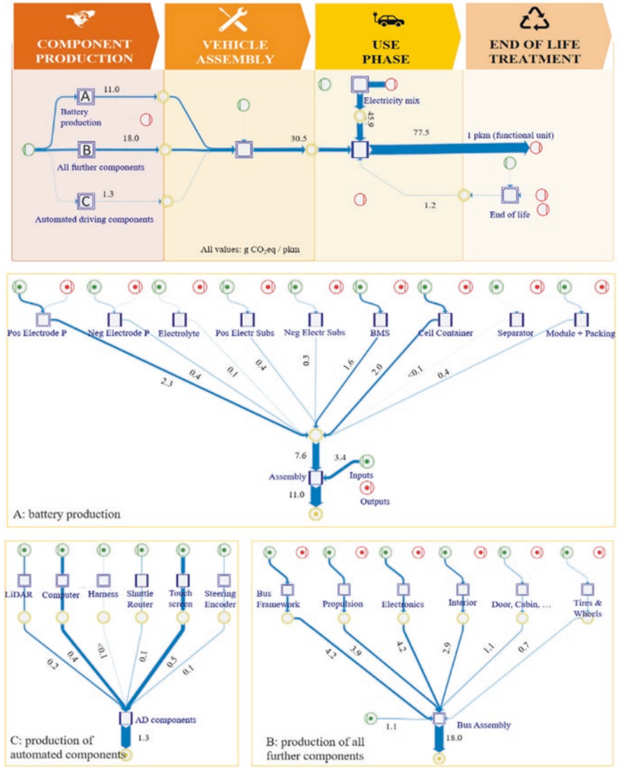
Fig. 13.2 Automated minibus life cycle model main model with subnets for battery production (a), production of all further components (b), and production of automated components (c). Sankey diagrams depict global warming potential in g CO 2 eq per pkM for the automated minibus near-future use case. In the Petri-net-based material flow network approach underlying the Umberto LCA software, blue squares represent processes or subnetworks, and circles represent input points (green), output points (red), and connection points (yellow). All values have been rounded to one digit
