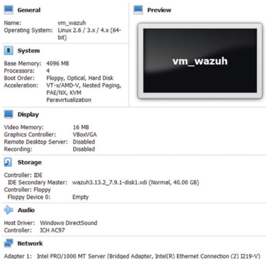
Fig. 7.6 Wazuh server VM specifications
