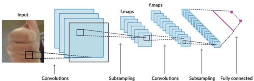
Fig. 5.18 CNN architecture for thumb orientation detection
