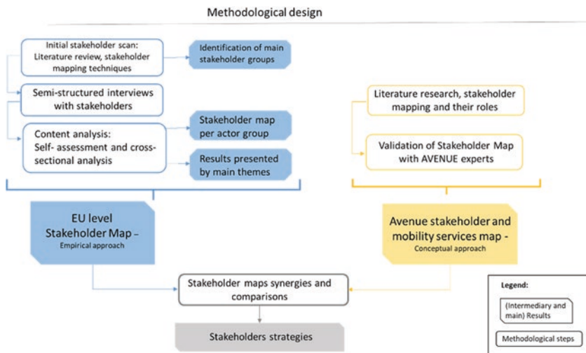
Fig. 9.1 Methodological approach
