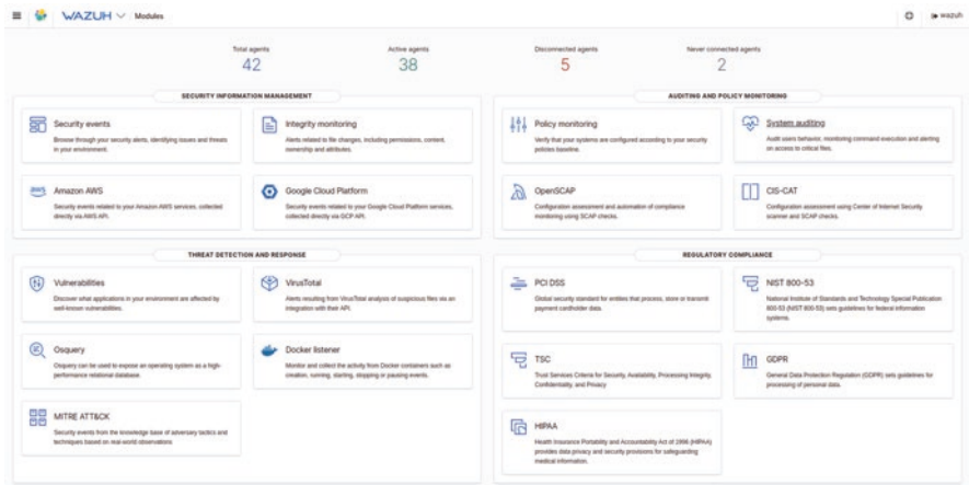
Fig. 7.8 Wazuh user interface modules
