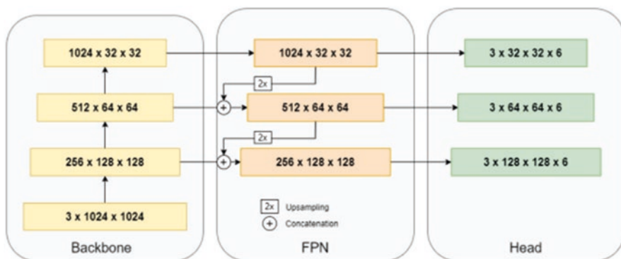
Fig. 5.12 An illustration of multiple convolutional layers and multidimensional matrices, such as the feature maps with 1024 \times 1024 input resolution (Tsiktiris et al., 2022)
