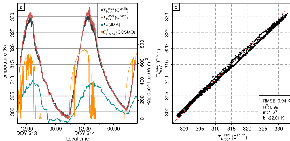
Figure 9. Inter-camera comparison of the mean broadband longwave radiation derived from roof pixels within the FOV of both cameras shown as (a) brightness temperatures ( T_{broof}^{cam} ) for C^{south} (black) and C^{north} (red) surfaces with observations at 1 min resolution.
