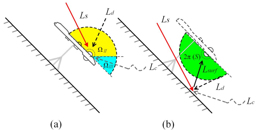
Figure 6. Radiative flux components of a slope-parallel positioned radiometer over a sloped surface in terms of the (a) incidence and (b) reflection. L_s , L_d , L_c and L_{surf} are the direct, sky, adjacent slope-reflected, and target slope-reflected radiance, respectively.
