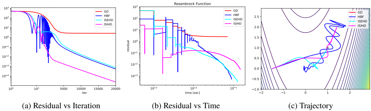
Figure 1: Results on the Rosenbrock function with \beta = 0.02 .
