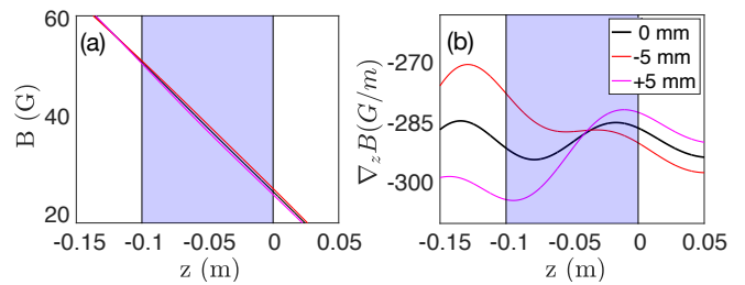
FIG. 3. Theoretical magnetic field (a) and gradient (b) for Case g^* = 0.65 , evaluated at different coil 1 vertical positions. The original coil position (black); 5 mm downwards (red); and 5 mm upwards (magenta) are shown.
