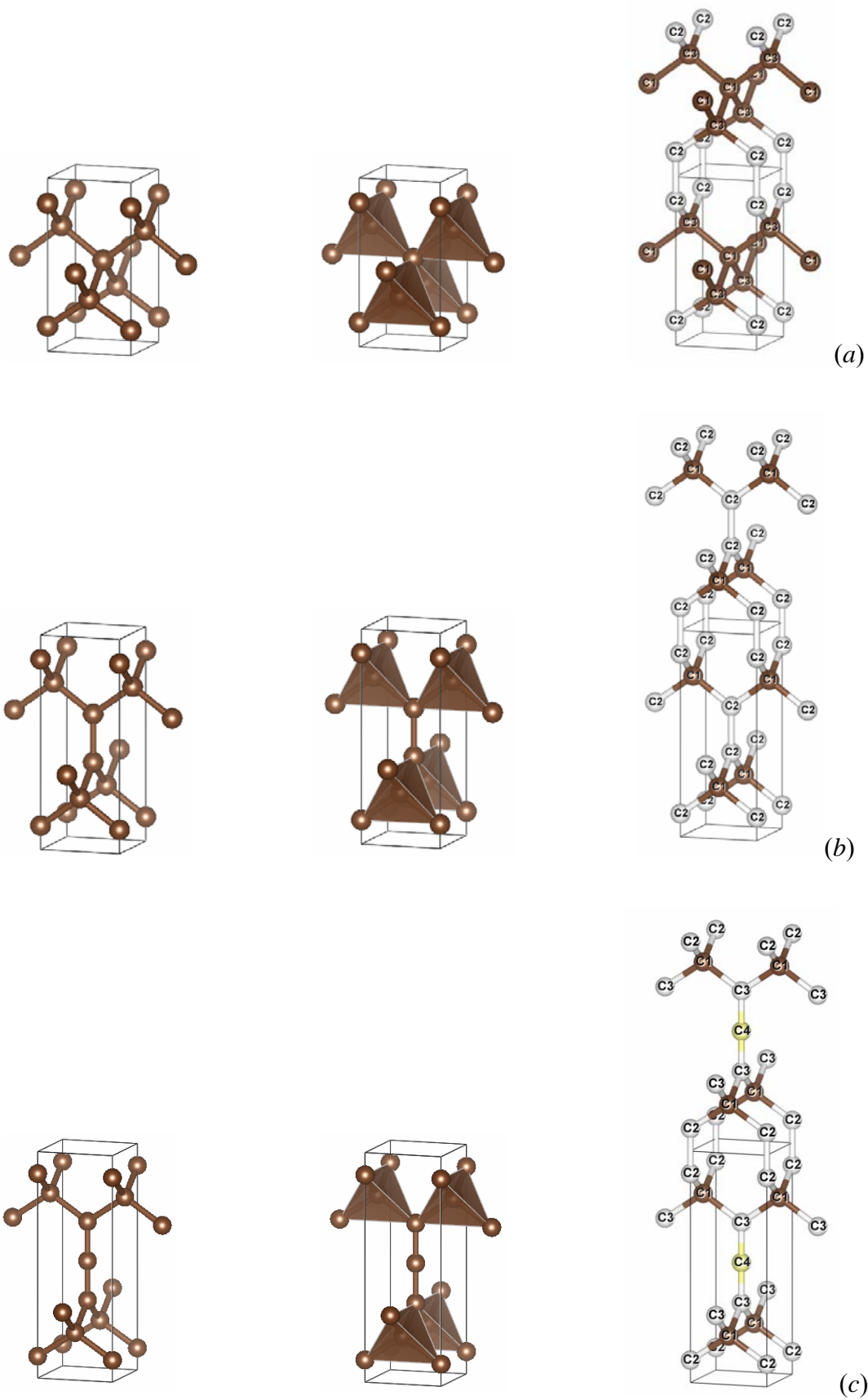
Figure 2 Crystal structures of new tetragonal carbon allotropes in three representations: ball-and-stick (left), polyhedral (middle), and double cells with atoms numbering as in Table 2: C 5 (a); C 6 (b); C 7 (c).
