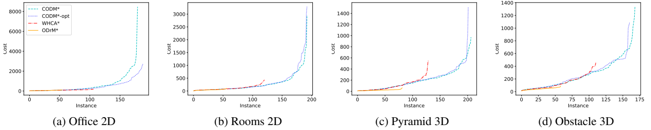
Figure 11: Cactus plots of costs for the algorithms in the case with connectivity, vertex, and swapping conflicts.
