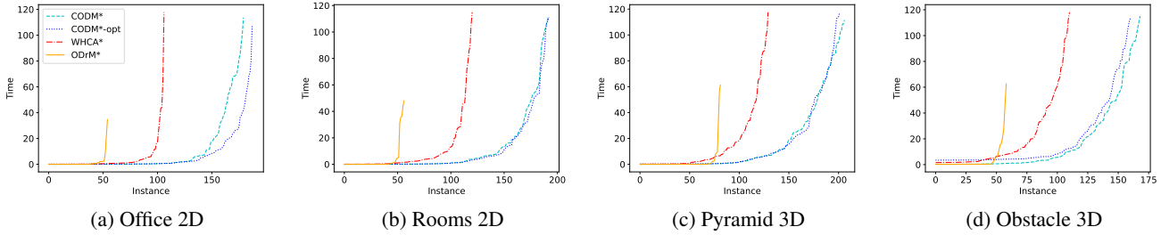
Figure 9: Cactus plots of executions times for the algorithms in the case with connectivity, and vertex with swapping conflicts. Each point (x, y) in the graph of an algorithm means that x benchmarks were solved each within y seconds. Thus a graph that is lower than the other means the algorithm is faster.
