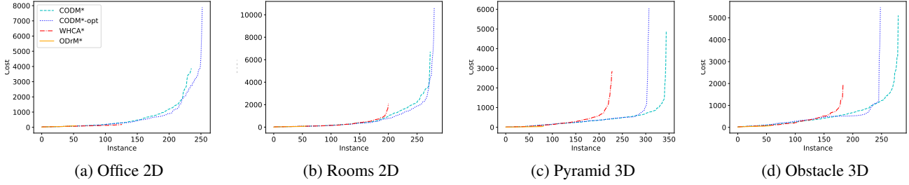
Figure 10: Cactus plots of costs for the algorithms in the case with connectivity, and vertex conflicts only. Each point (x, y) in the graph of an algorithm means that x benchmarks were solved providing an execution with makespan y (which is the size of the longest path). Thus a graph that is lower than the other means that the algorithm finds shorter executions.
