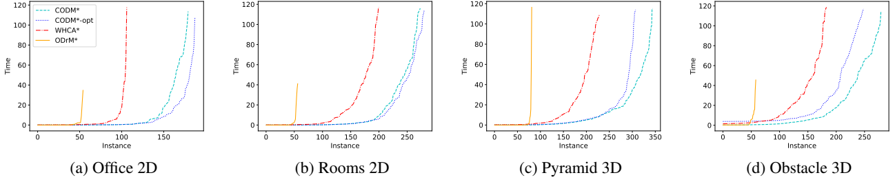
Figure 8: Cactus plots of executions times for the algorithms in the case with connectivity, and vertex conflicts only. Each point (x, y) in the graph of an algorithm means that x benchmarks were solved each within y seconds. Thus a graph that is lower than the other means the algorithm is faster.
