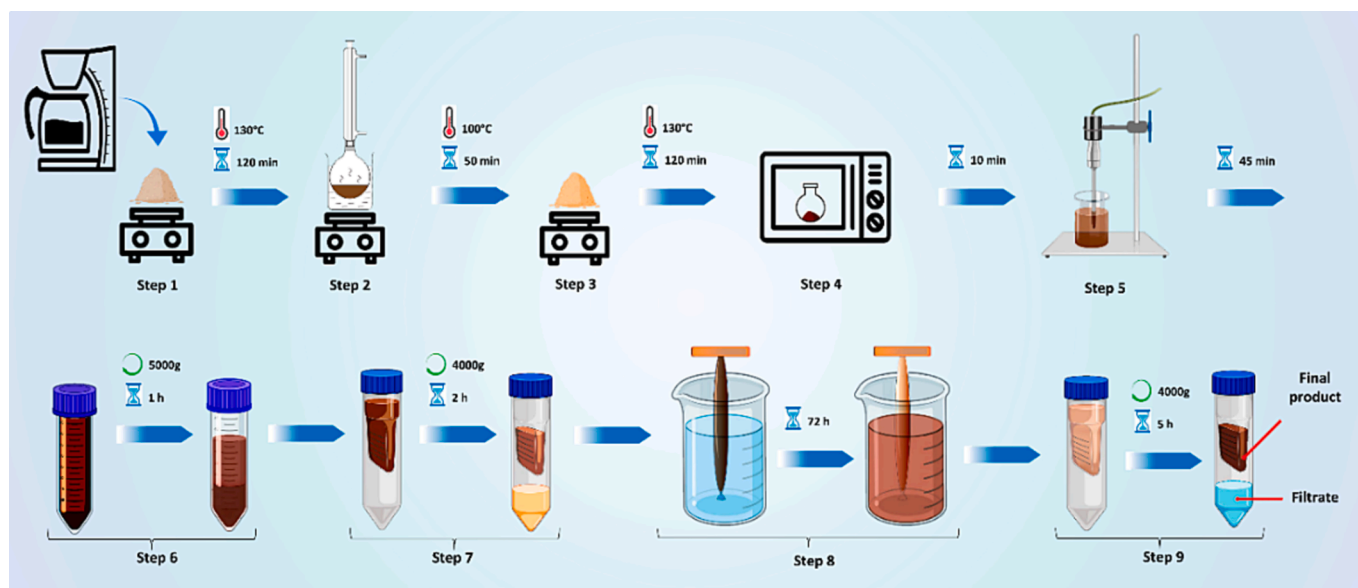
Fig. 1. Fabrication scheme of the coffee-based nano hybrids. Step 1 – Preliminary drying; Step 2 – Preliminary treatment and incorporation of Gd; Step 3 – Drying; Step 4 – Carbonization; Step 5 – Sonication; Step 6 – Debris elimination; Step 7 – Elimination of large nanoparticles; Step 8 – Dialysis; Step 9 – Pre-concentration.
