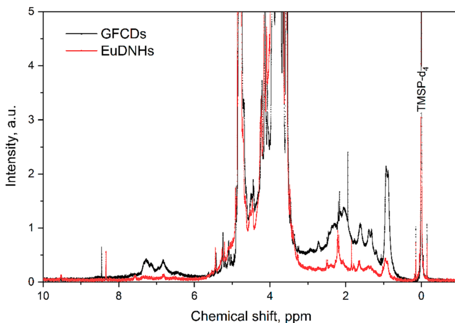
Fig. 6. ^1\text{H} NMR spectra of GFCDs and EuDNHs dispersed in \text{D}_2\text{O} . TMSP-d4 is used as a reference compound. Transmitter frequency – 400 MHz, fid resolution – 0.24 Hz.
