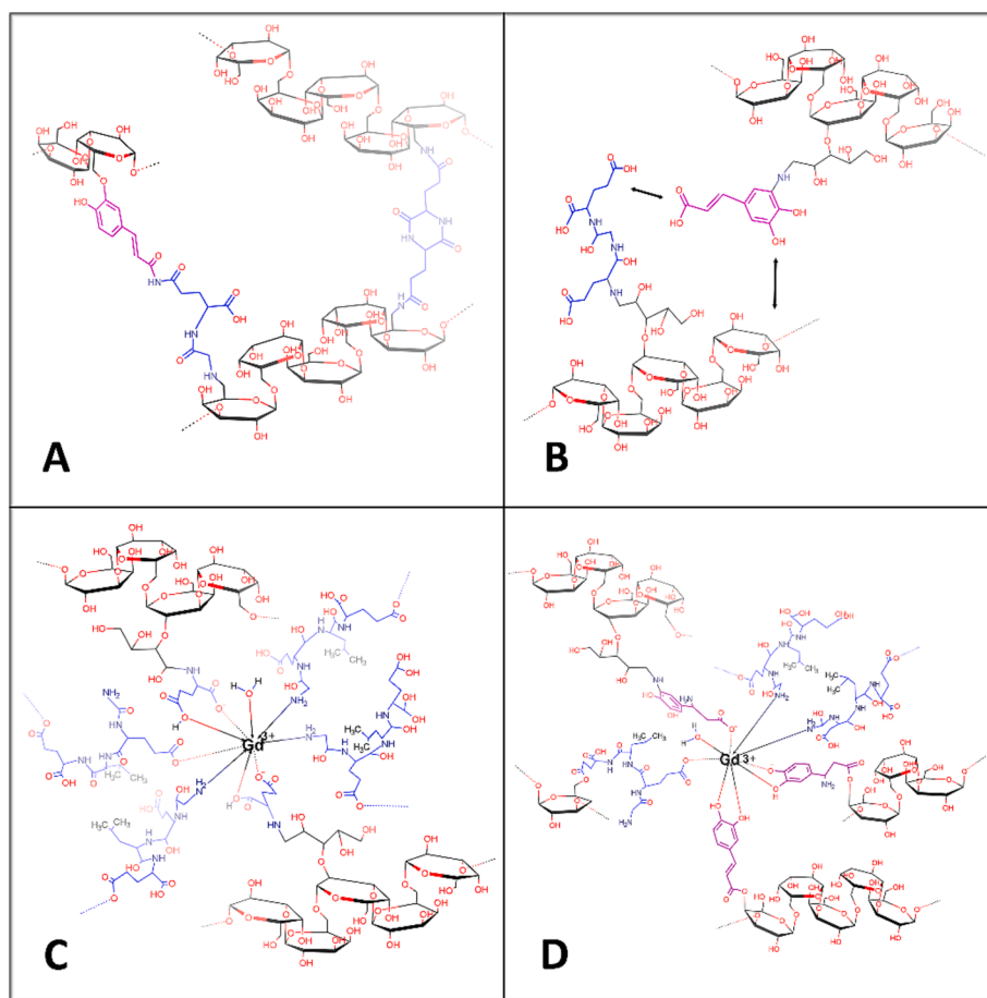
Fig. 9. Possible chemical formations in the \text{Gd} -free carbon dots associated with inner cross-linking (A) and repulsion (B). Specific domains in the \text{Gd} -doped nanohybrids participate in chelation of \text{Gd}^{3+} ions through amino acidic binding (C) and with hydroxycinnamic acid derivatives chelation (D). The drawings were made in Marvin Sketch v23.2, ChemAxon ( http://www.chemaxon.com ).
