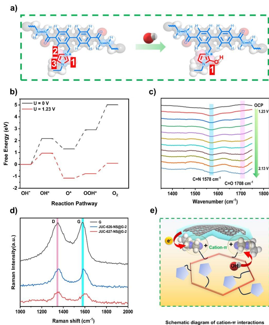
Figure 4. (a) Adsorption of \text{OH}^- on C1 atom of JUC-627-NS molecular fragment. (b) Free energy diagram for JUC-627-NS at U = 0 \text{ V} (black) and U = 1.23 \text{ V} (red). (c) In-Situ FT-IR spectra of JUC-627-NS at 1.23 V-2.13 V. (d) In-Situ Raman spectra of graphene (G), JUC-626-NS@G-2 and JUC-627-NS@G-2. (e) Schematic diagram of cation- \pi interactions promoting charge transfer.
