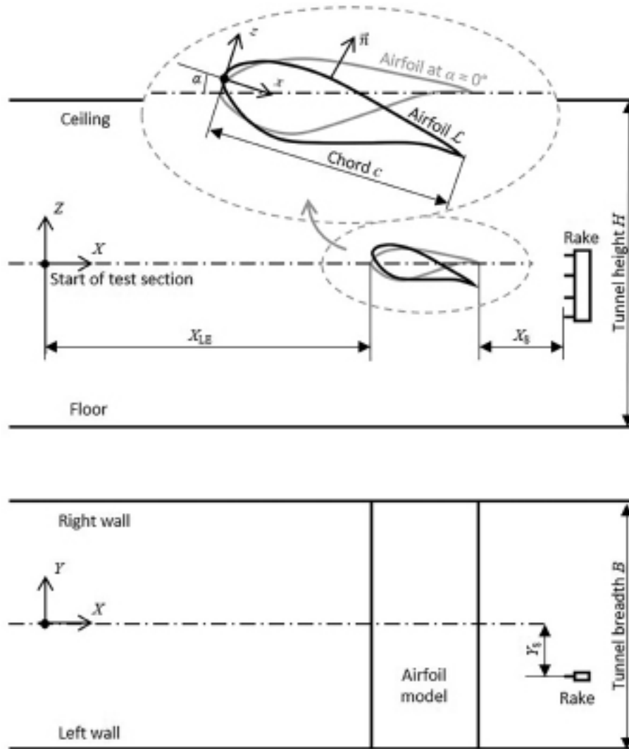
FIGURE 2 | Schematic of the wind tunnel experiment, with main geometrical notations indicated.
