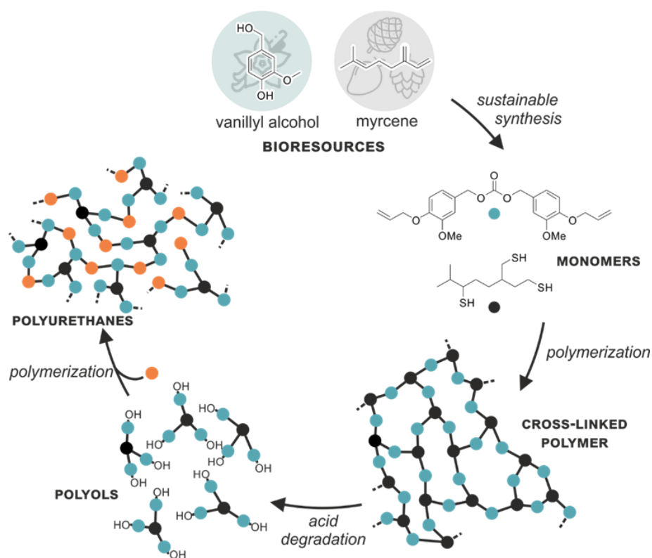
Figure 1. General strategy implemented in this study.
