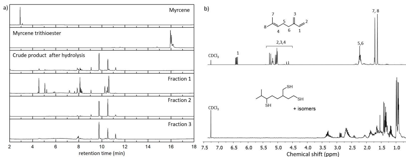
Figure 3. (a) GC-MS monitoring of the synthesis of myrcene trithiol, from the top to bottom: starting material myrcene, reaction mixture after reaction with thioacetic acid for 23 h, crude product after thioester hydrolysis, fraction 1, fraction 2 and fraction 3 collected after column chromatography, (b) ^1\text{H} NMR spectra of myrcene (top) and fraction 2 (bottom) in \text{CDCl}_3 .
