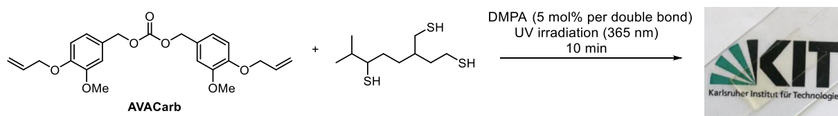
Figure 4. Thiol-ene coupling between AVACarb and myrcene-based trithiol resulting in a cross-linked polymer film (picture).
