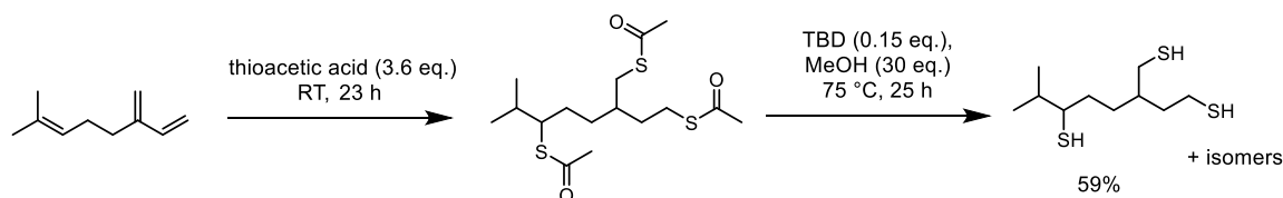
Scheme 2. Reaction scheme of the synthesis of myrcene trithiol monomer.
