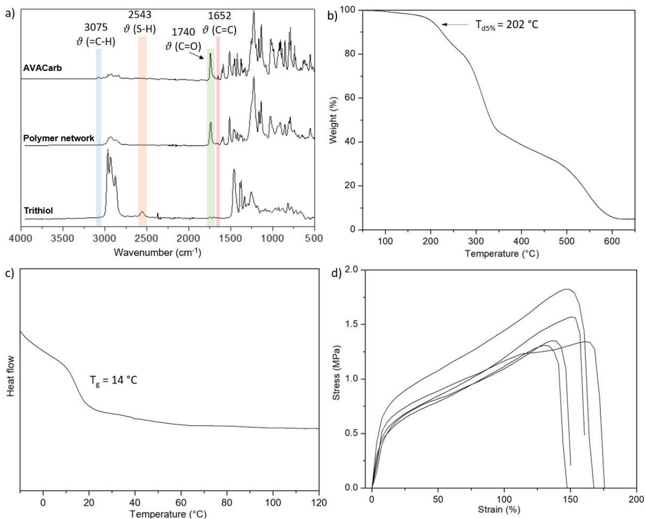
Figure 5. (a) FTIR spectra of myrcene trithiol (bottom), AVACarb (top) and resulting film (middle); (b) TGA thermogram, (c) DSC thermogram, (d) tensile tests (5 replicates), of polymer films obtained by thiol-ene polymerization of myrcene trithiol and AVACarb .
