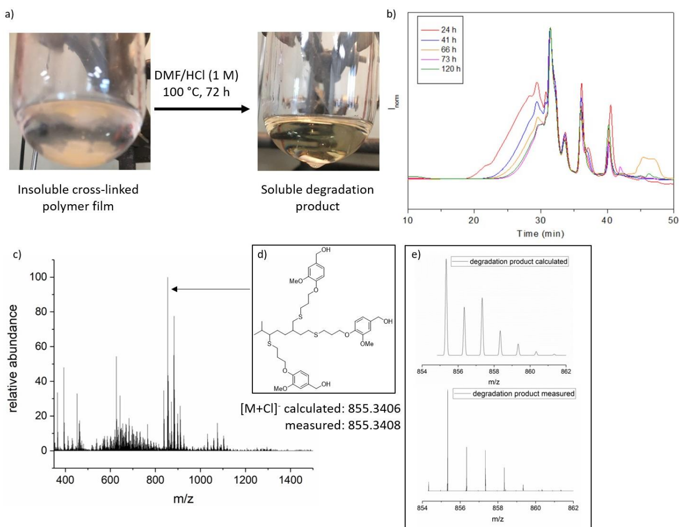
Figure 7. (a) Visual observation of the cross-linked polymer solubilization under degradation conditions, (b) SEC monitoring of the solubilized polymer, (c) ESI-MS spectrum of degradation product, (d) Chemical structure of the expected main degradation product, (e) calculated isotopic pattern (top), measured isotopic pattern of the expected degradation product.
