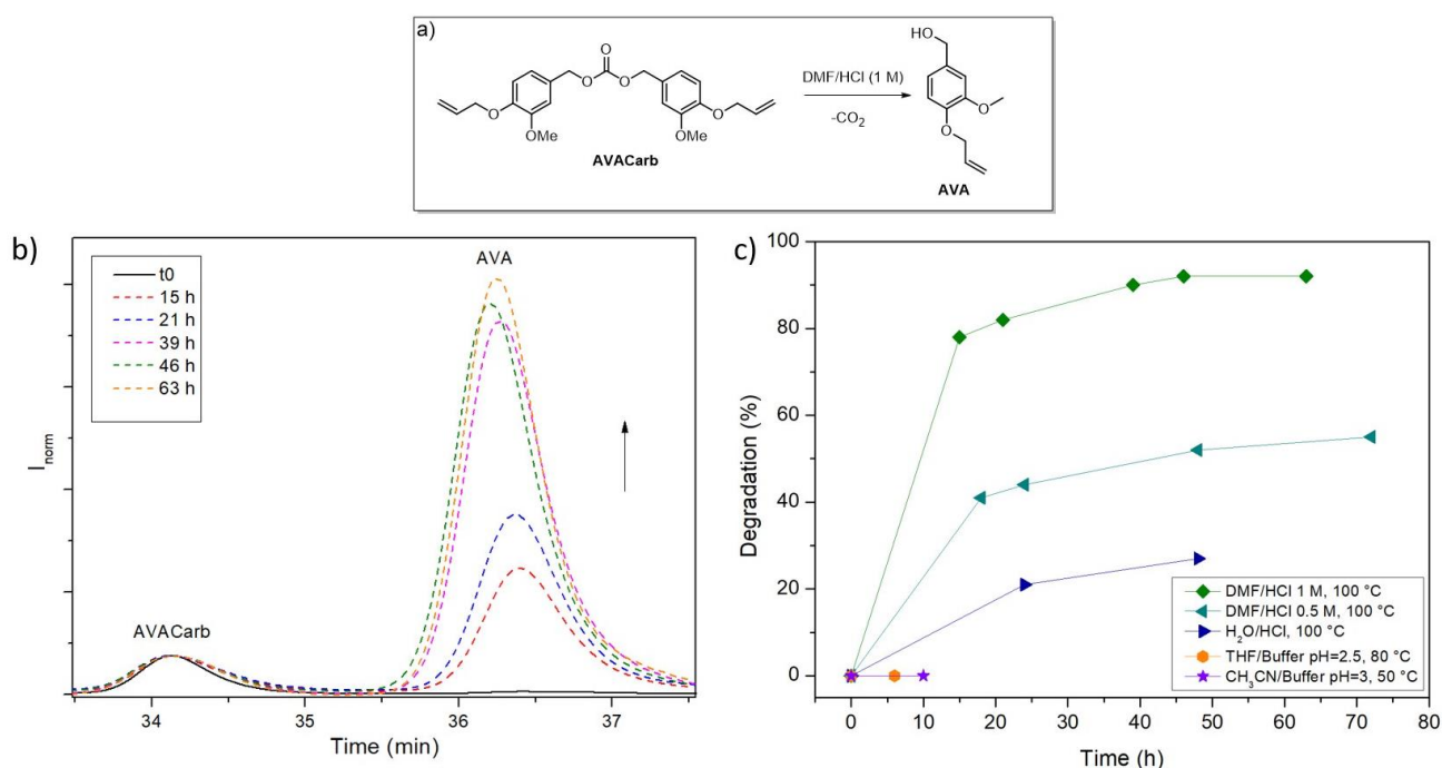
Figure 6. (a) Molecular model: cleavage of AVACarb into AVA under acidic conditions, (b) monitoring of the degradation in DMF/HCl 1 M at 100 °C via SEC, (c) establishment of degradation conditions for AVACarb : test of different reaction conditions.
