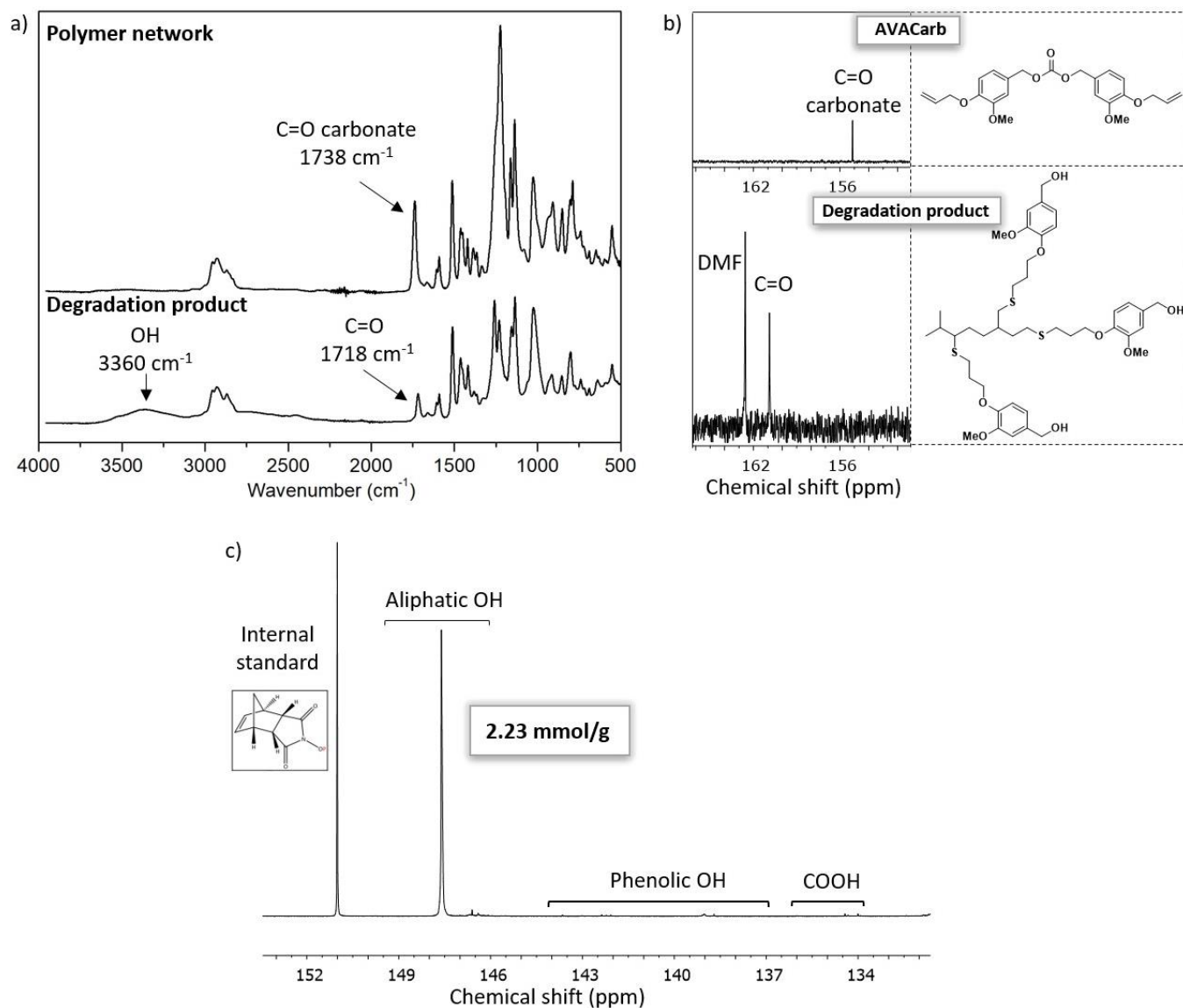
Figure 8. (a) FTIR spectra of the polymer network (top) and degradation product (bottom), (b) zoom on the ^{13}\text{C} NMR spectra of the AVACarb (top) and degradation product (bottom), (c) ^{31}\text{P} NMR spectrum of the phosphorylated degradation product.
