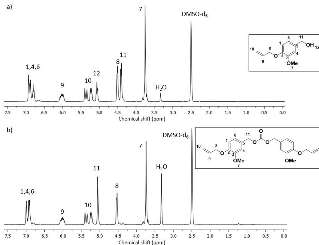
Figure 2. ^1\text{H-NMR} spectra of allylated vanillyl alcohol AVA (a) and the cleavable \alpha,\omega -diene AVACarb (b) in \text{DMSO-d}_6 .
