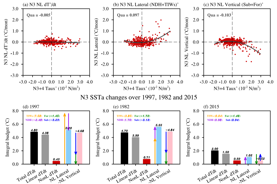
Figure 4. Scatterplot of Ni3 average mixed layer heat budget nonlinear terms (red dots; °C/month) as a function of Ni3 + 4 average zonal wind stress anomalies (Taux', 10 -2 Nm -2 ): (a) mixed layer temperature tendency (dT'/dt), (b) lateral contributions (sum of NDH and Tropical instability waves (TIWs)), (c) vertical contributions (sum of the subsurface and air-sea fluxes). Quadratic fits are indicated as gray lines on panels (a)–(c), with the quadratic coefficient indicated on the top left of each panel. Contributions to December minus January Sea Surface Temperature (SST) anomalies for panel (d) 1997, (e) 1982 and (f) 2015: total SST change (black) and contributions from linear (gray) and nonlinear (red) oceanic processes. The nonlinear contribution is further broken into lateral (blue, comprising TIWs in orange and NDH in purple) and vertical (pink, multiplied by -1 , comprising subsurface in blue and air-sea fluxes in green). The positive (negative) values are indicated by upward (downward) arrows.
