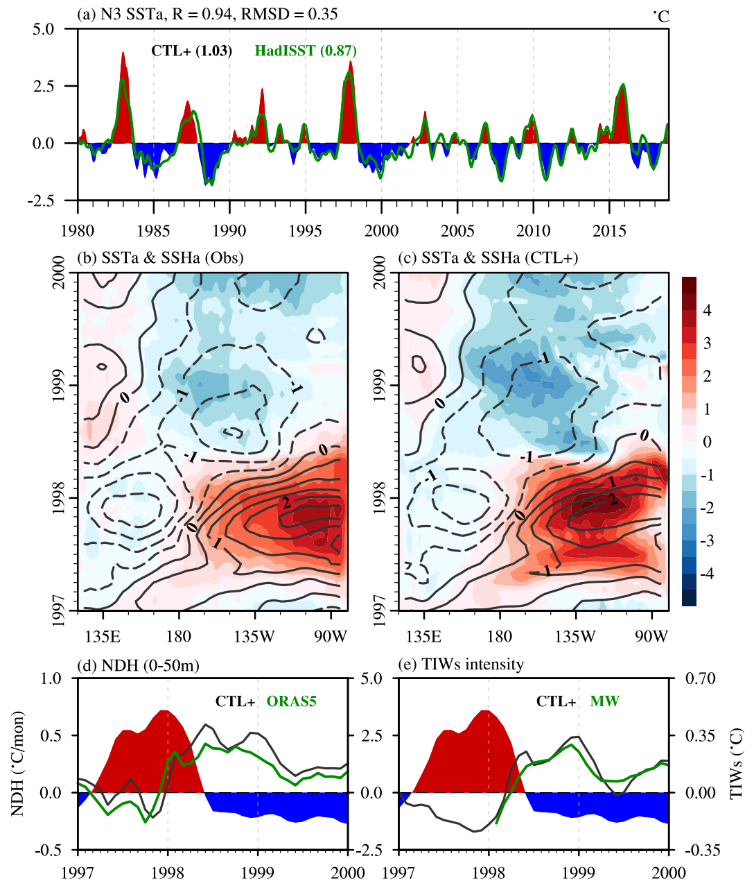
Figure 2. (a) Time series of Niño3 average Sea Surface Temperature (SST) anomalies for the CTL+ ocean simulation (red and blue shading; °C) and HadISST (green curve; °C). The number in brackets indicate the standard deviation of each curve, and their correlation and root mean square difference (RMSD) are indicated above. (b) Time-longitude section of observed SST (shading; °C) and SSH (contour; m) anomalies during 1997–1998. Panel (c) as panel (b), but for CTL+. (d) Time series of Niño3 average SST anomalies (red and blue shading; °C), 0–50 m average horizontal Nonlinear Dynamical Heating (NDH) in CTL+ (black curve; °C/month) and ORAS5 (green curve; °C/month). Panel (e) as panel (d), but for the CTL+ (black curve; °C) and Microwave OISST (green curve; °C) Tropical Instability Waves (TIWs) intensity index (see Section 2). A 3-month smoothing is applied to panels (a), (d) and (e).
