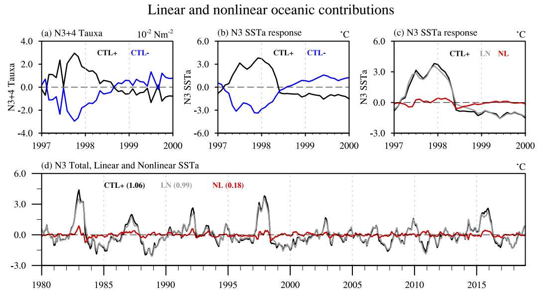
Figure 3. 1997–2000 time series of (a) Niño3 + 4 (5°S–5°N, 160°E–90°W) average zonal wind stress anomalies ( 10^{-2} \text{ Nm}^{-2} ) from the CTL+ (black curve) and CTL– (blue curve) ocean simulations. Niño3 average sea surface temperature (SST) anomalies ( ^{\circ}\text{C} ) in (b) CTL+ (black curve) and CTL– (blue curve), (c) CTL+ simulation SST anomaly ( ^{\circ}\text{C} ; black curve), and its decomposition into the linear (gray curve) and nonlinear (red curve) components of the response to anomalous wind stress. The linear component is obtained from the half difference of CTL+ and CTL– and the nonlinear component from their half sum (see Section 4). Panel(d) as panel (c), but for 1980–2018. The numbers within brackets indicate the standard deviation of each curve.
