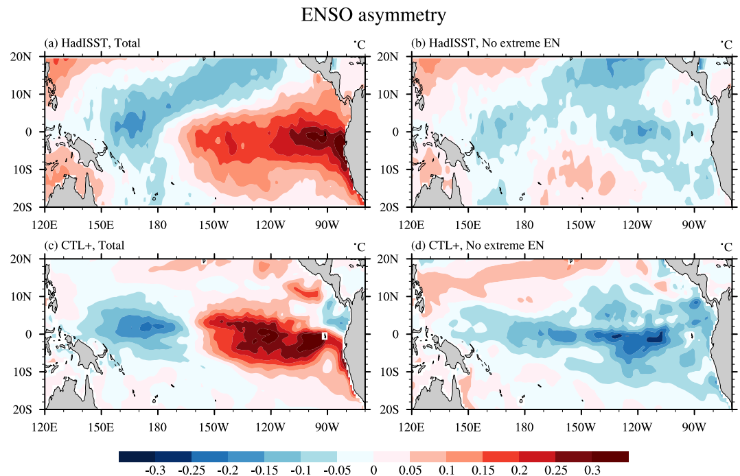
Figure 1. ENSO asymmetry (half sum of DJF El Niño and La Niña composites over 1980–2018, °C) for panel (a) HadISST and (c) the control ocean simulation CTL+, (b) and (d) as (a) and (c), but excluding the 1982, 1997 and 2015 extreme El Niño events from the asymmetry computation.
