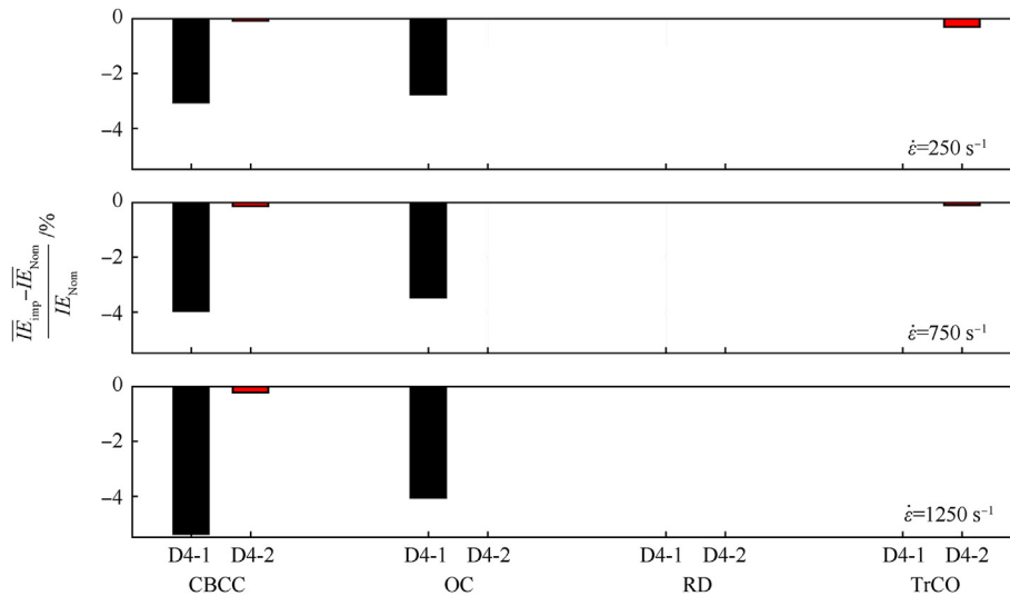
Fig. 14. Percentage error between \overline{E}_{Imp} and \overline{E}_{Nom} for all RVE geometries by considering scenarios D4-1 and D4-2 of Table 3 and \dot{\epsilon} = [250, 750, 1250] \text{ s}^{-1} .
