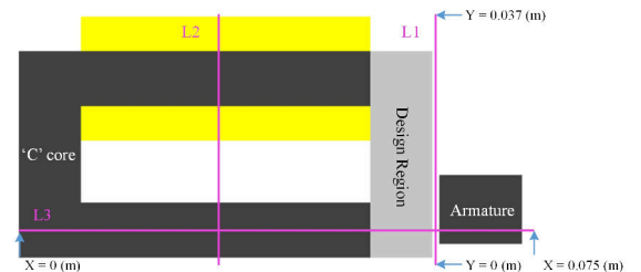
Fig. 14. The design region of the electromagnetic actuator
