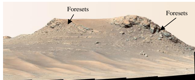
Fig. 1. ~14 m (left) and ~22 m (right) tall foresets at Pinestand Mountain (zcam08726)
