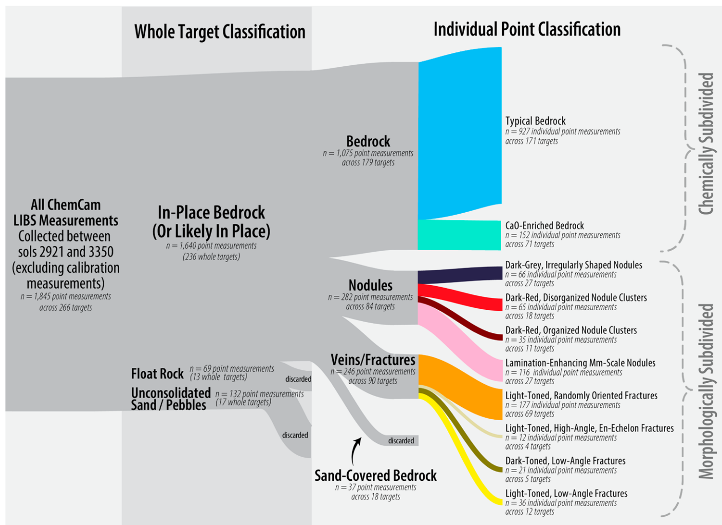
Figure 3. Classification scheme of ChemCam laser-induced breakdown spectroscopy (LIBS) data. See Figures S1-A1 through S1-A10 for examples of all classification schemes (see text footnote 1). All ChemCam LIBS data collected on geologic targets between sols 2921 and 3350 were included in initial analyses. Float rock and unconsolidated sand and pebble targets were differentiated from in-place bedrock measurements and discarded. Individual LIBS point measurements within each in-place bedrock ChemCam target were then further classified according to geologic feature sampled (bedrock, nodules, veins/fractures, and sand-covered bedrock), as apparent from ChemCam Remote Micro Imager (RMI) images. Sand-covered bedrock measurements were discarded. Bedrock measurements were then chemically subdivided into two subclasses, nodules were morphologically subdivided into four subclasses, and veins/fractures were morphologically subdivided into four subclasses, as recognized via Mastcam image analysis of near-field rover workspaces.
