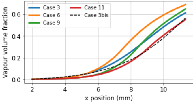
FIGURE 15: VAPOUR VOLUME FRACTION FOR THE DIFFERENT STUDIED CASES
