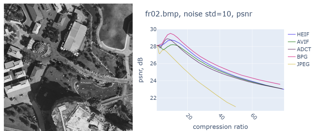
Figure 13. The test image Fr02 and dependencies PSNR tc (CR) for it, \sigma^2 = 100 .
