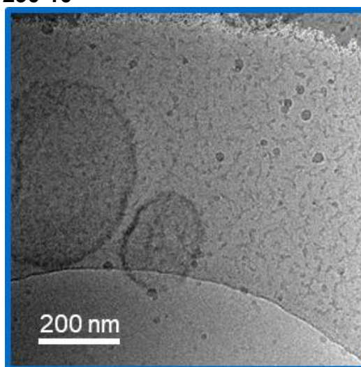
Figure 3. Impact of the M_n of the core block with constant AA content ( f_{AA,0} = 0.1 ): (top) Fitted SAXS data. The model used and dimensions are reported in Table S4 . (bottom) Representative cryo-TEM pictures of the samples.
