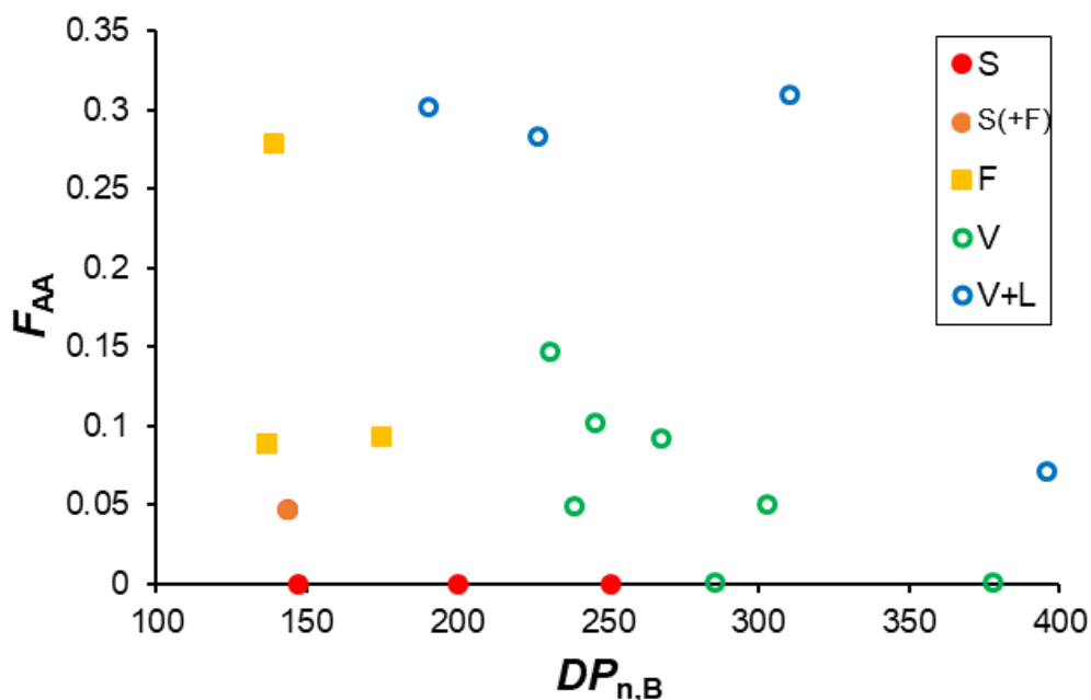
Figure 4. Summary of the experiments performed at natural pH ( \alpha \sim 0 ). The color indicates the final morphology obtained determined by SAXS and cryo-TEM. S = spheres, F = fibers, V = vesicles and L = lamellae.
