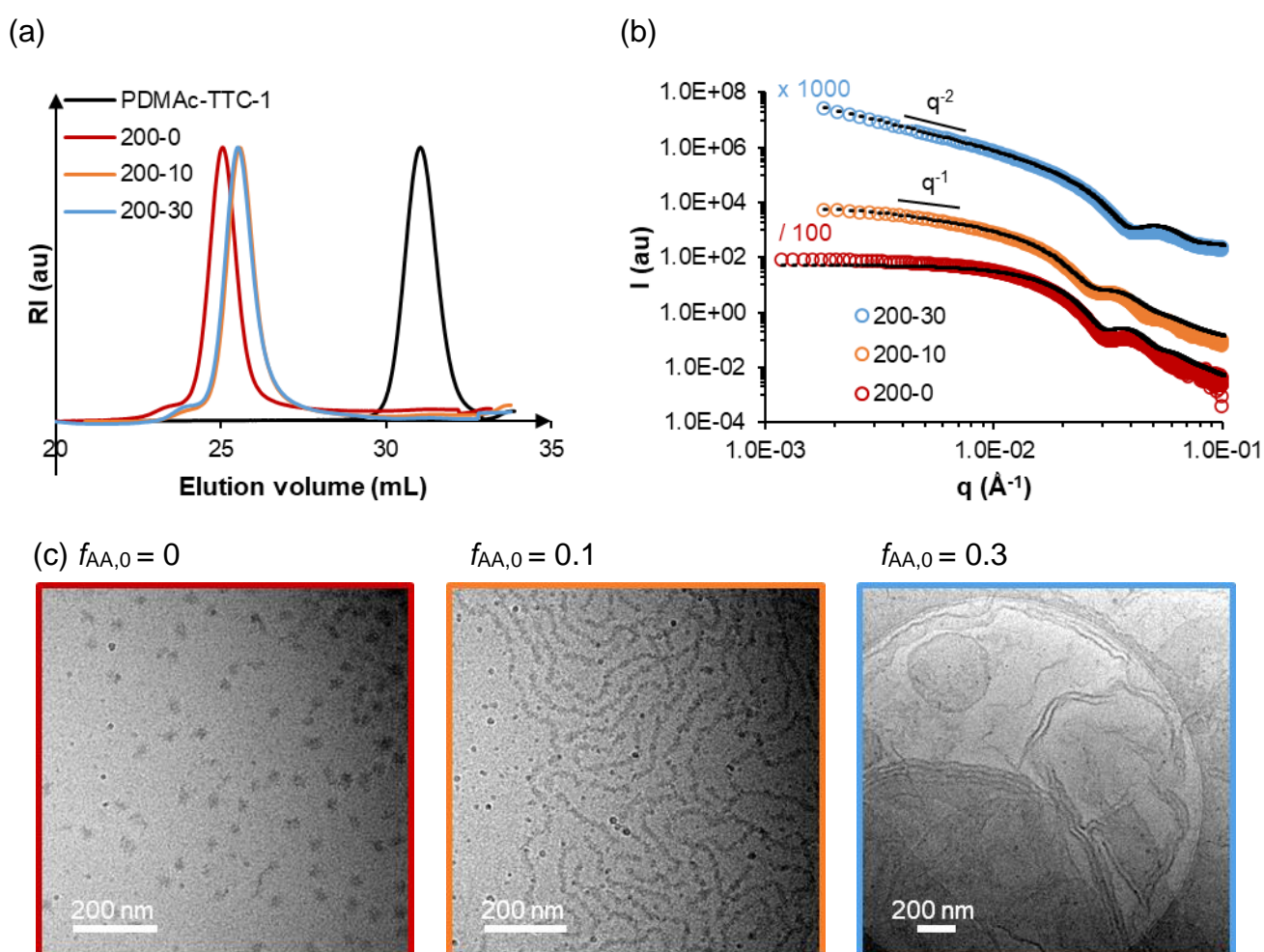
Figure 2. (a) SEC traces, (b) SAXS data and (c) cryo-TEM images of samples 200-0, 200-10, and 200-30 (samples synthesized with variable f_{AA,0} , and constant R \approx 200 ). The black dotted lines are models fitting the experimental data. The model used and dimensions are reported in Table S4 .
