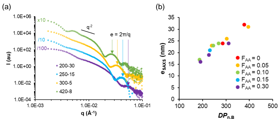
Figure 5. (a) SAXS data for typical lamellar objects with various DP_{n,B} . The arrows indicate that the membrane thickness, e , varies. Values of e reported in Table S4 were determined by fitting the data with a vesicle model. (b) Variation of e with the DP_{n,B} of the core block. e was determined by fitting SAXS data with a vesicle or lamellar model (see fitted SAXS data in Figure S6, and dimensions in Table S4).
