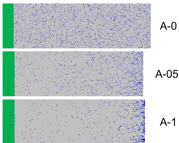
Figure 7. Simulation of 100 monodisperse PDMAc- b -P(MEA- co -AA) chains, stacked horizontally. The PDMAc block is represented in green, MEA in grey and AA units in blue. Each line on a figure corresponds to a different chain. The direction of polymerization is from left to right. Experimental f_{AA,0} , R , reactivity ratios of MEA and the final global conversion were used in the terminal model to determine the composition profiles (see SI, Figure S9 ). [46]
