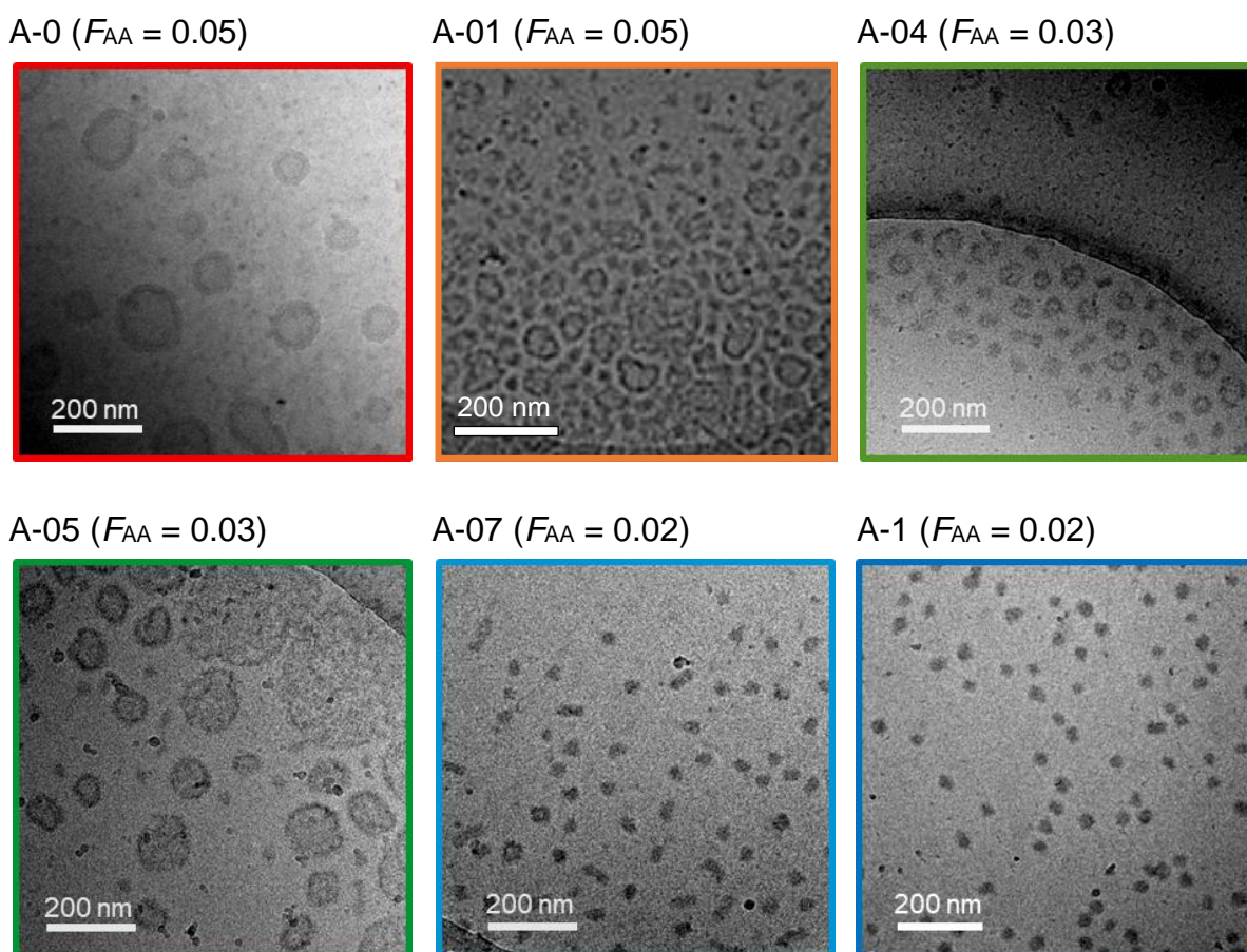
Figure 8. Representative cryo-TEM images ( C = 30 g/L) of samples of series A ( R = 300, f_{AA,0} = 0.05 , prepared by PISA at different \alpha_0 ).
