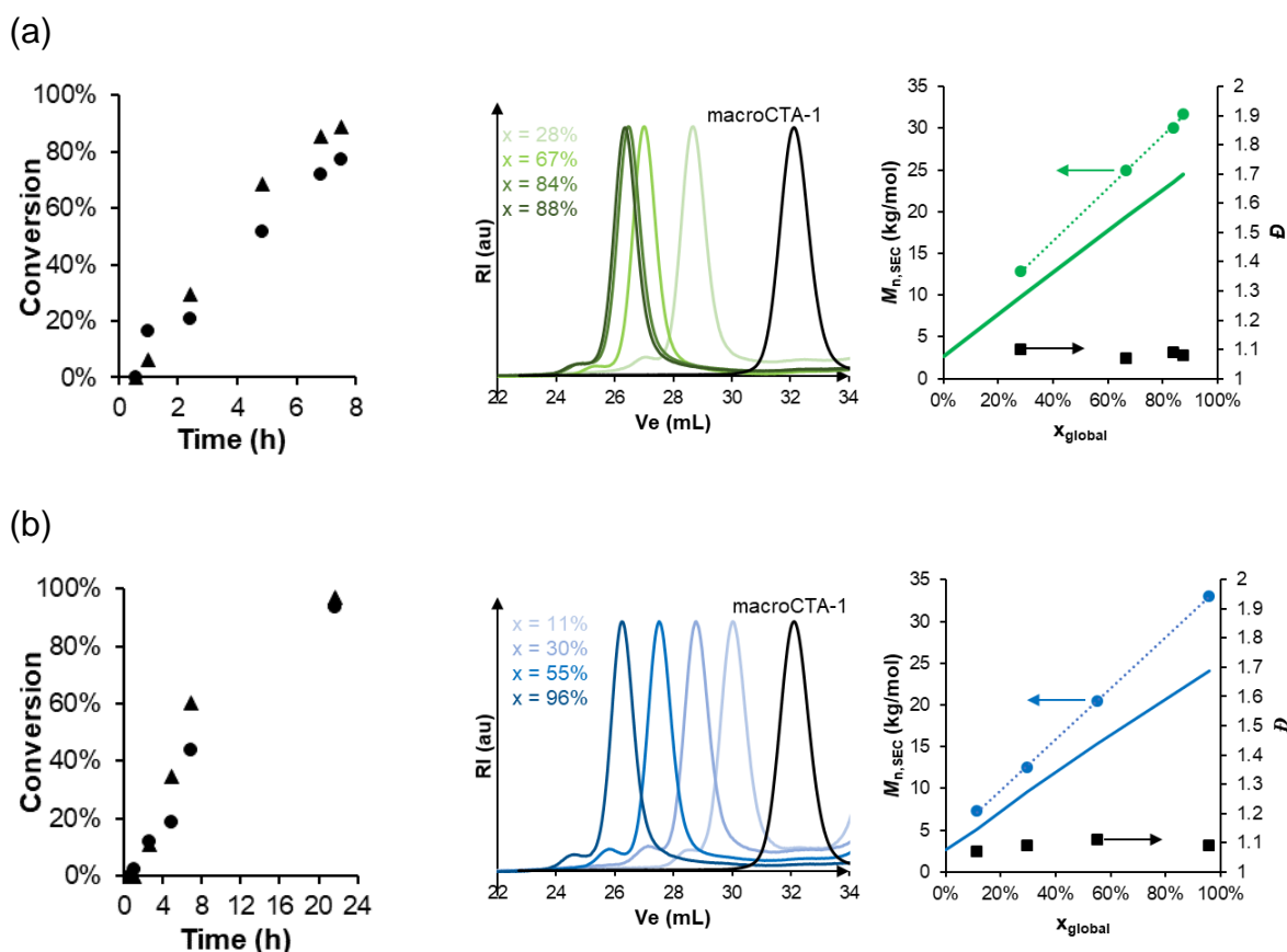
Figure 1. Kinetic monitoring of the aqueous dispersion copolymerization of MEA and AA in the presence of macroCTA-1 ( R \approx 200 ). (a) Sample 200-10 and (b) sample 200-30. (left) Individual conversion determined by ^1\text{H} NMR of MEA ( \blacktriangle ) and AA ( \bullet ). (middle) Overlay of the normalized SEC RI traces. The global monomer conversions, x , are indicated in the insert. V_e stands for elution volume. (right) Number-average molar mass, M_n , and dispersity, D , determined by SEC with PMMA calibration. The solid line shows the theoretical molar mass.
