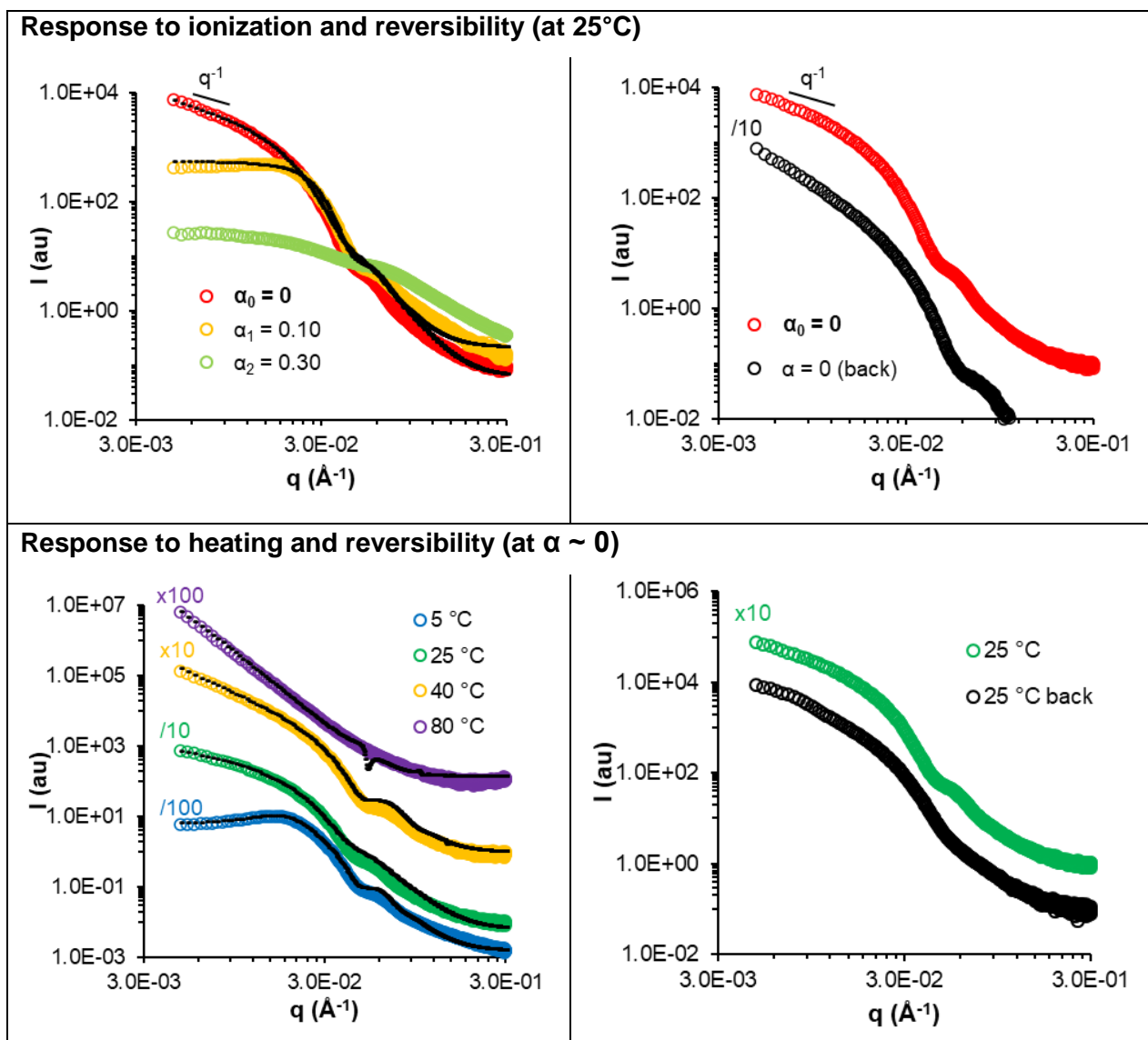
Figure 11. SAXS monitoring of the response of sample 150-30 ( short fibers ) to progressive deprotonation at 25 °C (top) and temperature (bottom, at \alpha \sim 0 ) ( C = 50 g/L). The black dotted lines are models fitting the data (see Table S7 and S8 ).
