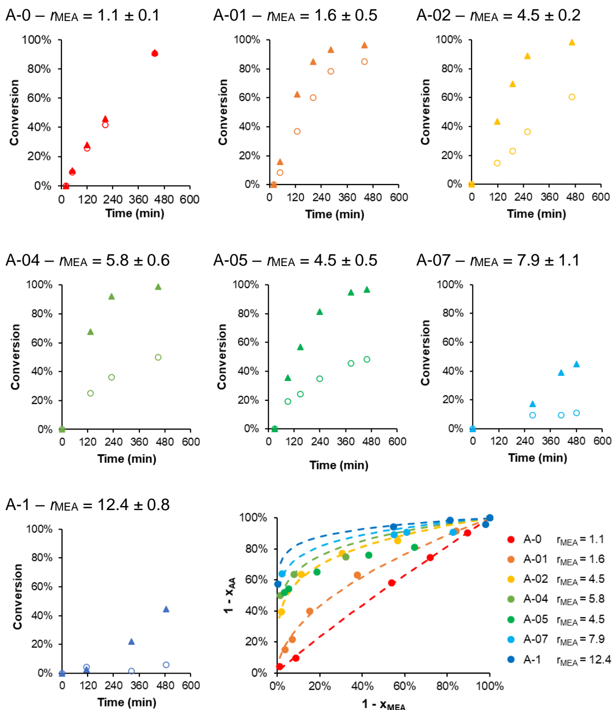
Figure 6. Kinetic monitoring of PISA conducted at different \alpha_0 (samples A-0 to A-1, with R = 300 and f_{\text{AA},0} = 0.05 ) displaying the individual conversions in MEA (▲) and AA (○). Jaacks plot showing the fitting curves in dotted lines. A-0 corresponds to sample 300-5.
