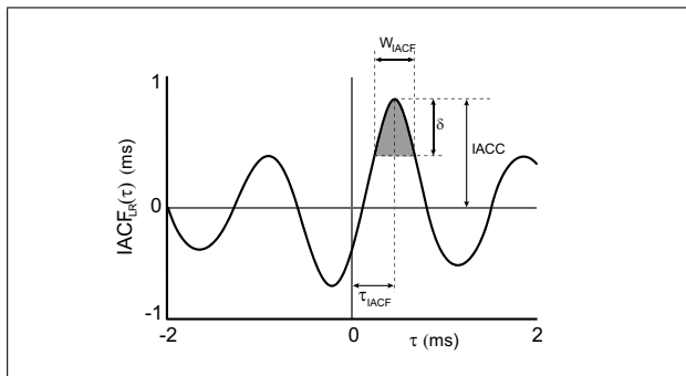
Figure 5. InterAural Cross-correlation Function (IACF) and schematic definitions of IACC, W_{IACF} and \tau_{IACF} .
