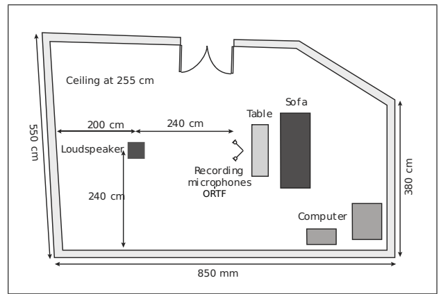
Figure 1. Recording set-up and listening room configuration.
