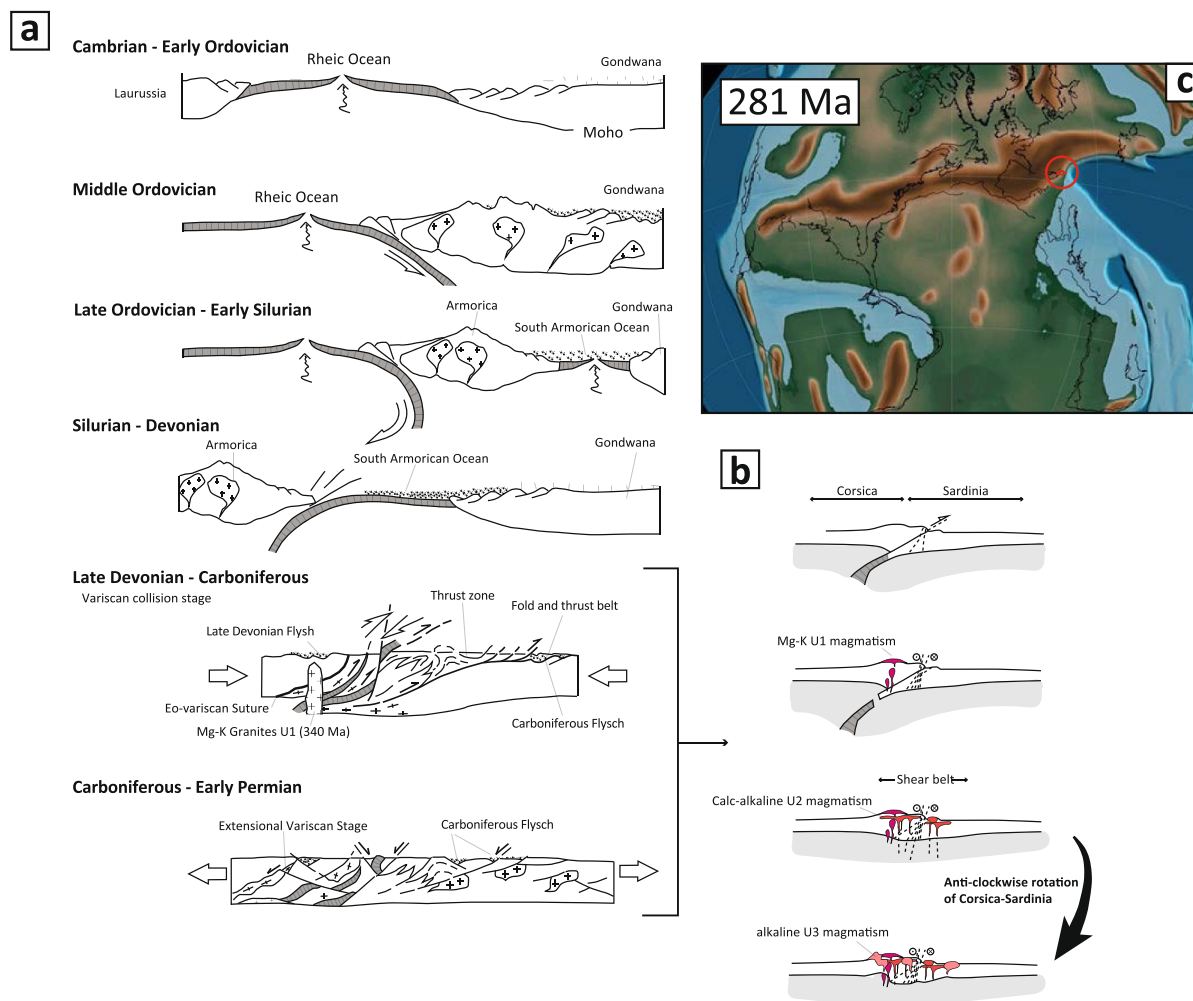
Figure 2. (a) Schematic diagrams of the geodynamic evolution of the Corso-Sardinian block during the Paleozoic (Rossi et al., 2010). (b) Geodynamic evolution of the Corsica-Sardinia block in Variscan times (Casini et al., 2015). (c) Panafrican and Eo-Variscan contact reconstruction where Corsica is located on the equator line and circled in red (Scotese & van der Pluijm, 2020).
