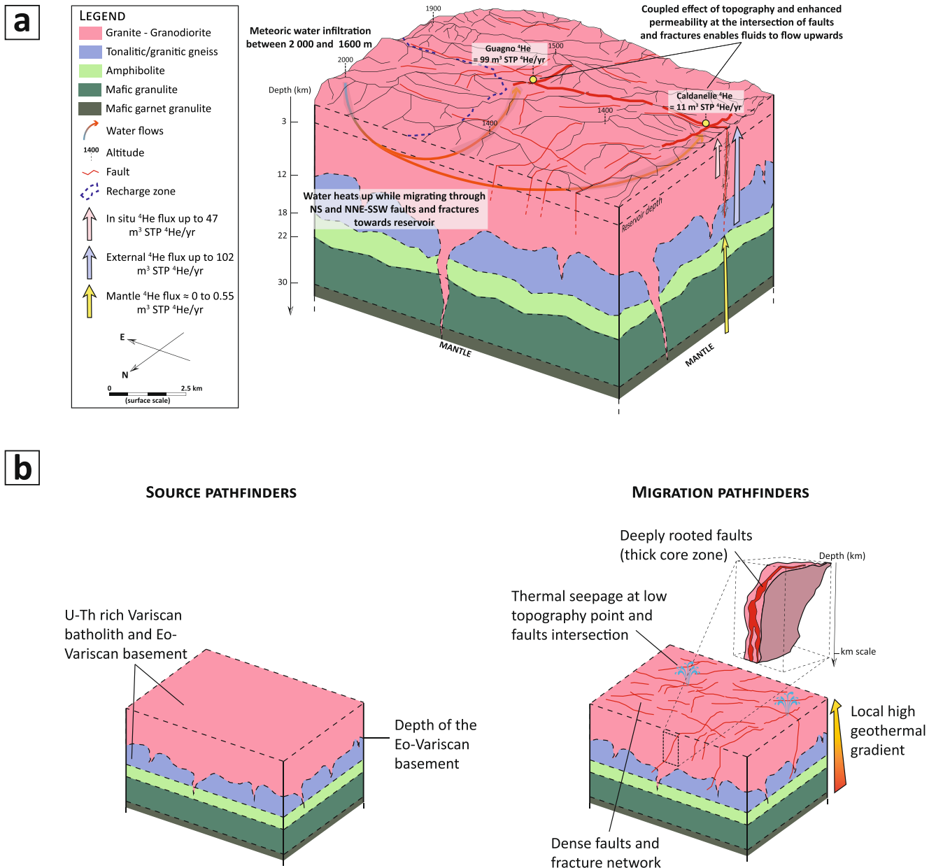
Figure 12. (a) schematic 3D block summarizing the thermal system of Caldanelle and Guagno-Les-Bains thermal springs and showing the source, migration and escape of helium. Layer geometry is not representative. (b) Schematic 3D block summarizing the source and migration pathfinders for helium exploration in a Variscan geological context.
