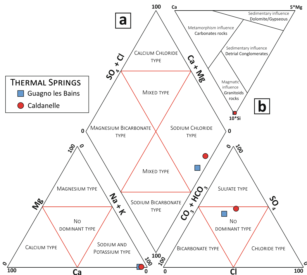
Figure 6. (a) Piper diagram, showing the main characteristic of the water chemistry of Caldanelle and Guagno springs. (b) Water-rock interaction ternary diagram (Derron & Pfeifer, 2018; Guggenbach, 1988) showing that the chemical profiles of the studied waters are consistent with circulation through a granitic basement.
