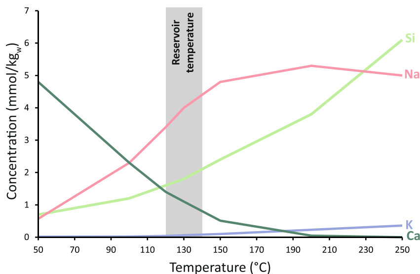
Figure 7. Concentrations of Si, Na, K, and Ca of a Na-Cl bearing water (5 mmol/kg w NaCl) equilibrated with primary and secondary minerals typical of granite hydrothermal alteration (see text) at temperatures ranging from 50 to 250°C. The modeled concentration of these elements matches the one measured at Caldanelle and Guagno for temperatures ranging from 120 to 140°C (gray area).
