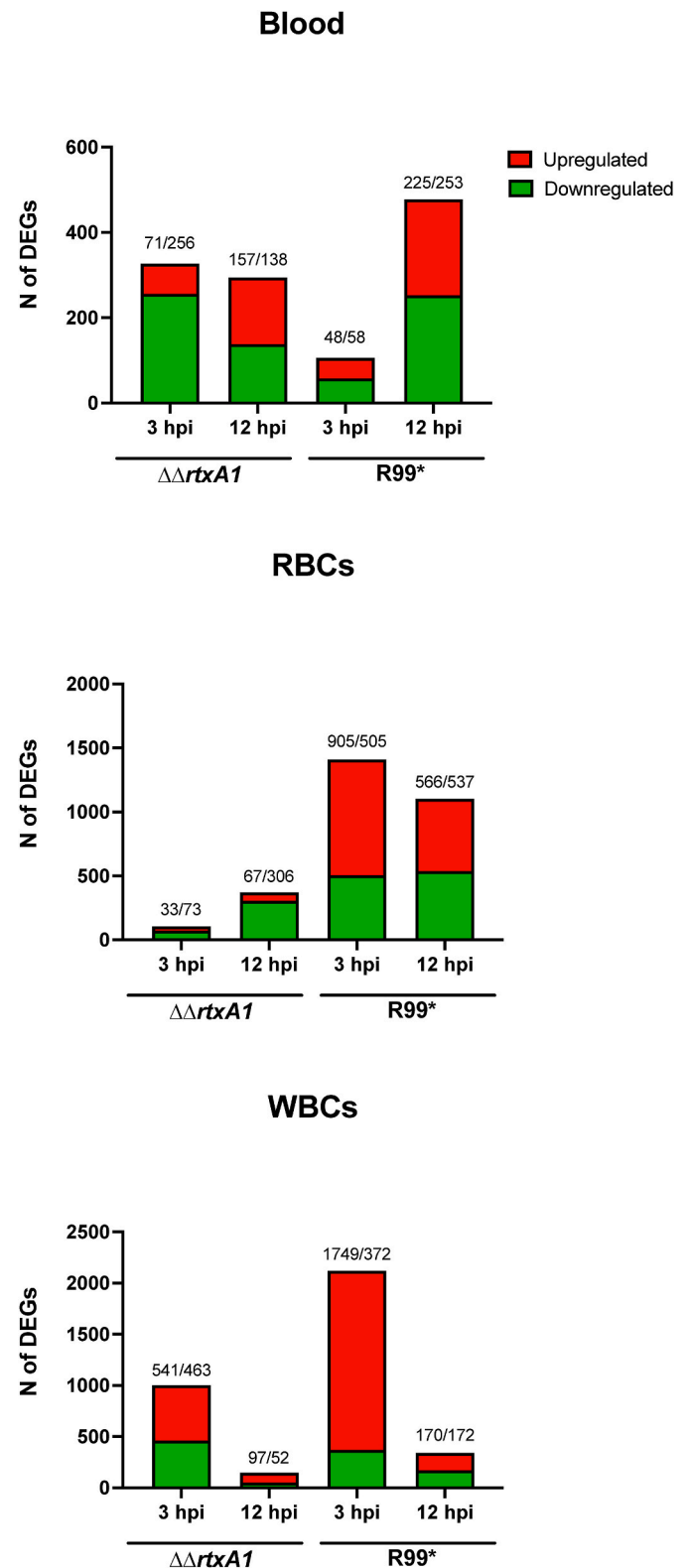
Fig. 1. Magnitude of the eel blood immune response against toxin-producing (R99) and non-toxin-producing ( \Delta\Delta rtxA1 ) V. vulnificus . Bars represent the total number of differentially expressed genes (DEGs; upregulated [red] or downregulated [green]) per sample (blood, RBCs [red blood cells] and WBCs [white blood cells]) and sampling time relative to time 0. The numbers of up-/downregulated DEGs are indicated at the top of each bar. * Data for infection with the parental toxin-producing strain (R99) were taken from Hernández-Cabanyero et al., [7].
