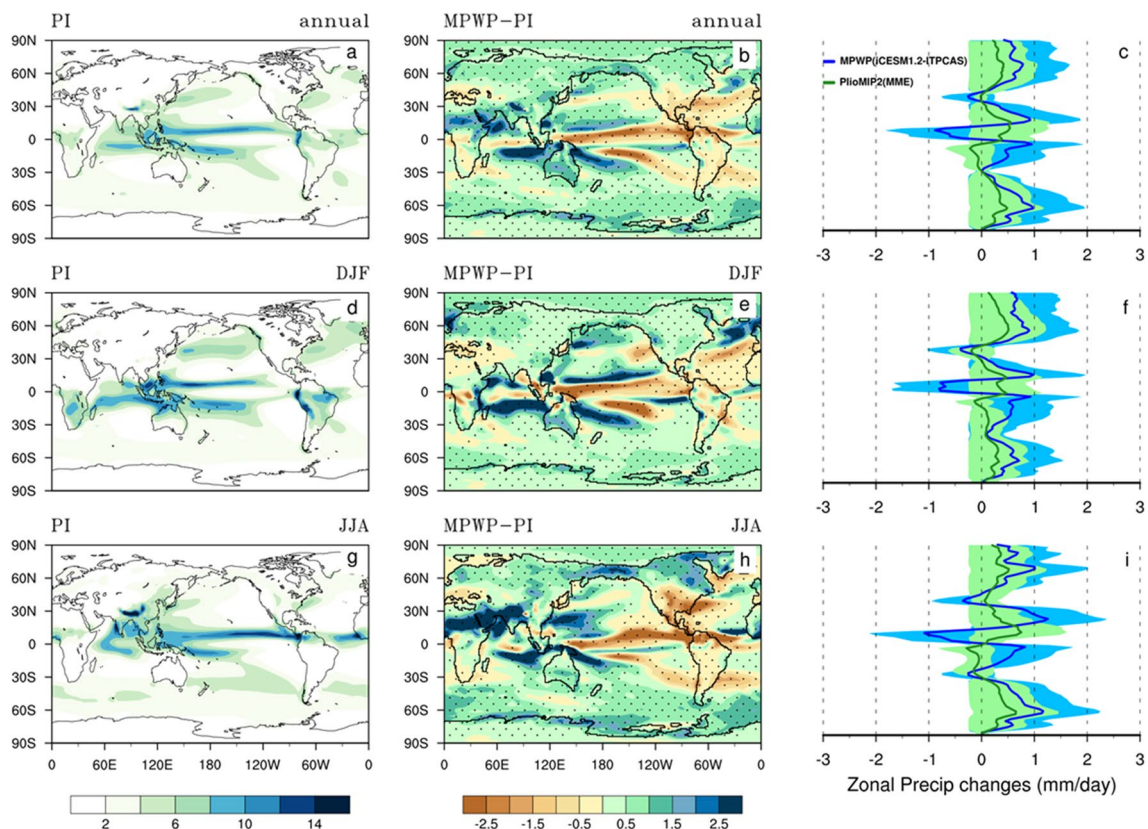
Fig. 5 As in Fig. 2, except for precipitation (mm/day). The right panel shows differences in the meridional gradient of precipitation for iCESM1.2-ITPCAS (blue) and PlioMIP2 multi model ensemble
