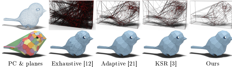
Fig. 3: Comparison with Plane Arrangements. Our algorithm builds a more concise plane arrangement than existing mechanisms (top row), leading to a polyon mesh with fewer facets (bottom row).
