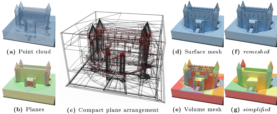
Fig. 2: Pipeline. Our method processes a set of planes with their corresponding inlier points (b) detected from a point cloud (a) into a compact plane arrangement (c). From this arrangement we extract either a watertight and intersection-free surface mesh (d) or a volume mesh with intersection-free convexes (e). The surface mesh can optionally be remeshed to represent each planar region with only one facet, and with Delaunay triangles for regions with holes (f). The remeshed surface is still watertight and intersection-free. The volume mesh can be simplified by merging groups of convex volumes and potentially allowing them to intersect (g).
