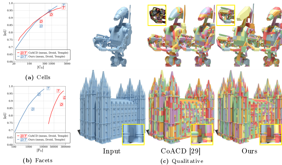
Fig. 6: Volume Decomposition with Non-Overlapping Convexes. We plot the volumetric IoU in function of the number of cells |C_V| (a) and facets |F_V| (b). Our algorithm offers a trade-off between IoU and number of convexes similar to the one of CoACD [29], but with convexes with fewer facets. In (c), the top row shows two decompositions for both methods of the Droid with different levels of complexity. The bottom row shows a decomposition of the Temple . For a similar number of convexes (colored cells), our algorithm captures the geometry better (see stairs on the bottom close-up), with fewer facets (see edges on the top close up).
