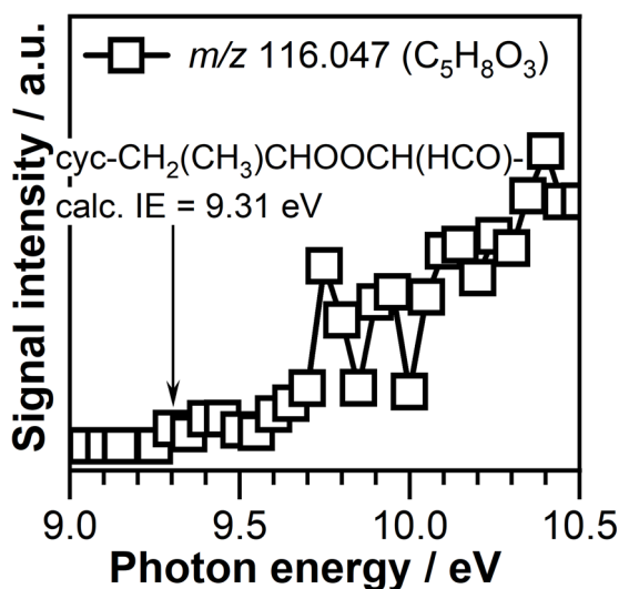
Fig. 11 Photoionization efficiency curve of m/z 116.047 ( C_5H_8O_3 ) signal measured at a temperature of 390 K. The arrow indicates the adiabatic ionization energy of the cyc\text{-}CH_2(CH_3)CHOOCH(HCO) compound.
