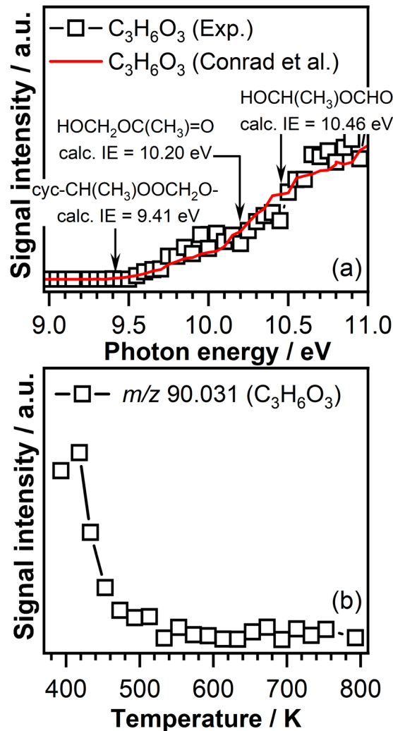
Fig. 6 (a) Photoionization efficiency curve of m/z 90.031 ( \text{C}_3\text{H}_6\text{O}_3 ) signal measured at a temperature of 390 K (open symbol) and compared with spectra from Conrad et al. (red curve). (b) \text{C}_3\text{H}_6\text{O}_3 signal intensity represented as a function of temperature recorded at a photon energy of 10.50 eV.
