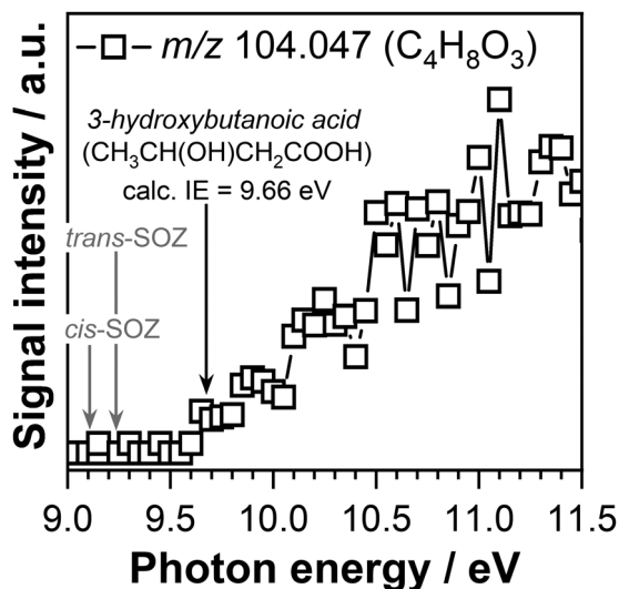
Fig. 7 Photoionization efficiency curve of m/z 104.047 (C 4 H 8 O 3 ) signal measured at a temperature of 390 K. The adiabatic ionization energy of 3-hydroxybutanoic acid calculated in this work is indicated with a black arrow. Gray arrows indicate the calculated adiabatic ionization energies of the cis -SOZ and trans -SOZ adopted from ref. 56.
