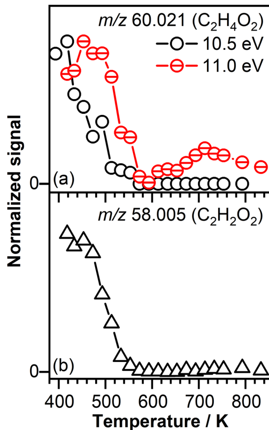
Fig. 5 (a) C_2H_4O_2 signal intensity represented as a function of temperature recorded at a photon energy of 10.50 eV and 11.00 eV, respectively. (b) C_2H_2O_2 signal intensity represented as a function of temperature recorded at a photon energy of 11.00 eV.
