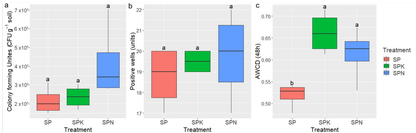
Figure 3. Boxplots representing the effects of applying two soil prebiotics on soil community-level physiological profiling (CLPP) measures compared to the control: (a) colony forming units (CFUs), (b) metabolic richness or number of positive wells (Units) with optical density ( OD > 0.25 ), and (c) metabolic activity or average well color development (AWCD), which is measured at 48 h (h) post plates' inoculation. SP plants without any treatment (control); SPK plants treated with K1 ® ; SPN plants treated with NUTRIGEO L ® . Each treatment is denoted by a color, where red is for SP, green is for SPK, and blue is for SPN. Data presented are means \pm SD. Bars labeled with the same letters within each graph indicate no significant difference ( p < 0.05 ) as determined using the ANOVA LSD test.
