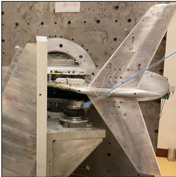
Figure 3-6 Static tests on the horizontal stabilizer
