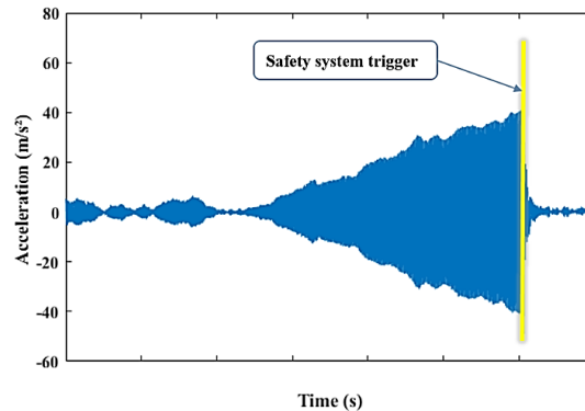
Figure 4-16 Accelerometer response during flutter onset
