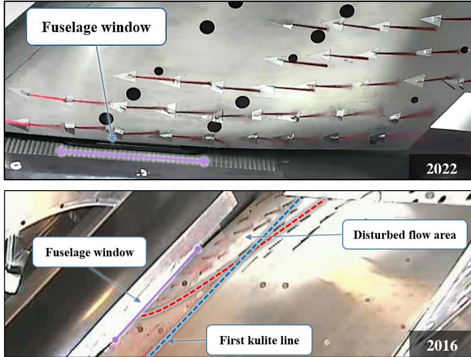
Figure 4-4 Wool tuft comparison between 2016 test and 2022, T=2^\circ , M=0.7 , P_i=1\text{bar} , AoA=0^\circ
