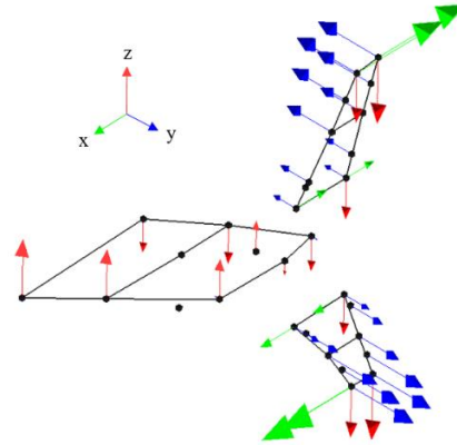
Figure 3-13 Second mode shape
