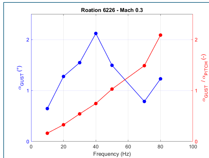
Figure 24 : Typical results of Movable flapped vanes gust generator for Mach = 0.3 (driving signal Frequency effect)
