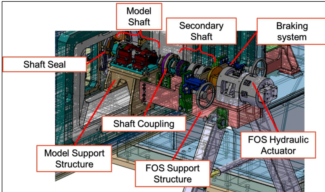
Figure 29 : WT model supporting structure assembly with all the main components
