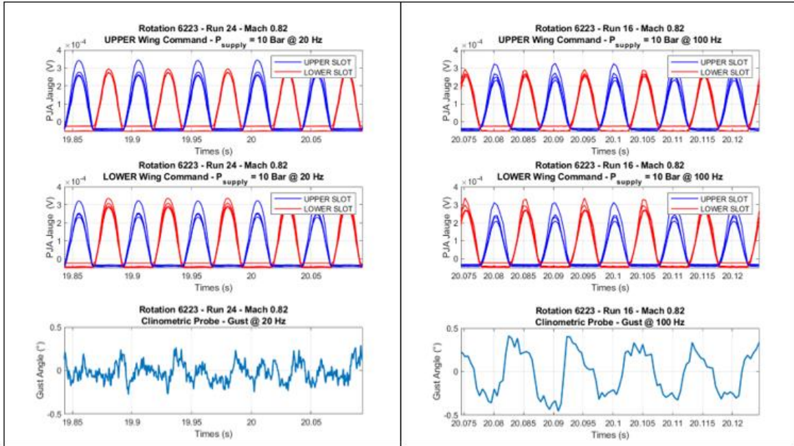
Figure 19 : Temporal evolution of Gust Generator Commands and Clinometric Probe Signal for tests at Mach = 0.82 and P_{supply} = 10 Bar
