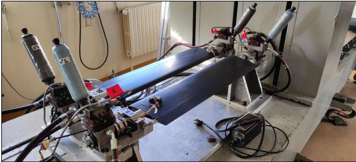
Figure 11 : Laboratory characterisation of the movable flapped vanes gust generator
