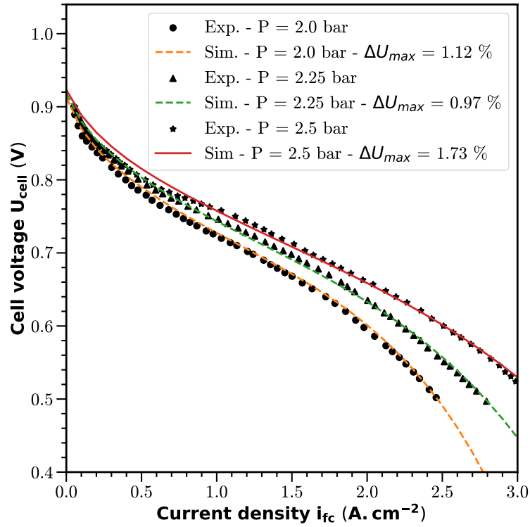
Figure 3: Polarization curves generated by AlphaPEM simulating a single fuel cell system from EH Group [24] under various operating conditions.
