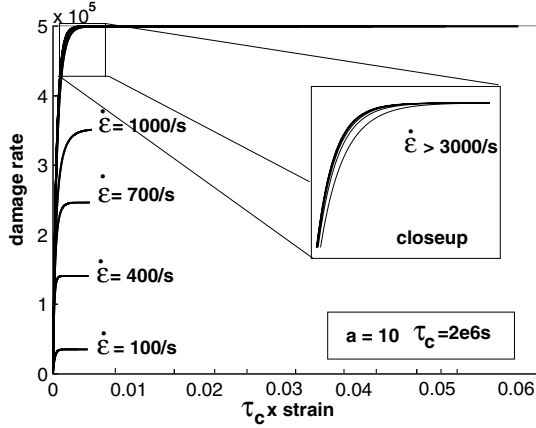
Fig. 8. Damage rate as a function of the strain; effect of the strain rate.
