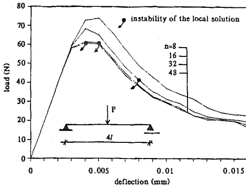
FIG. 8. Three-Point Bending; Convergence of Nonlocal Solution for Load-Deflection Curve
