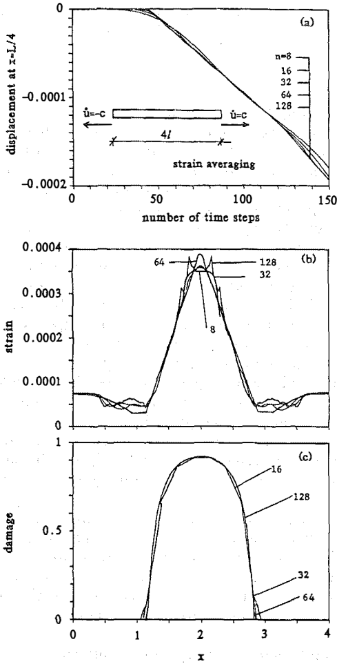
FIG. 9. Strain-Averaging Solution: (a) Convergence of Displacement History, (b), (c) Strain and Damage Profiles
