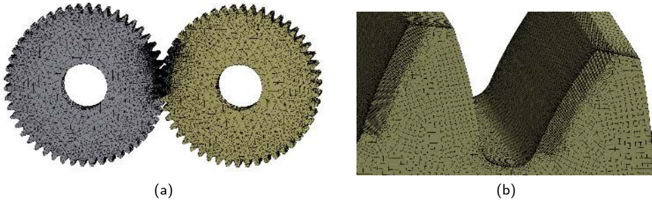
Figure 3: (a) the spur gear mesh with hexa-linear element at the tooth and tetra element elsewhere (b) close-up of the tooth mesh with 100 hexa-linear element and an inflation.
