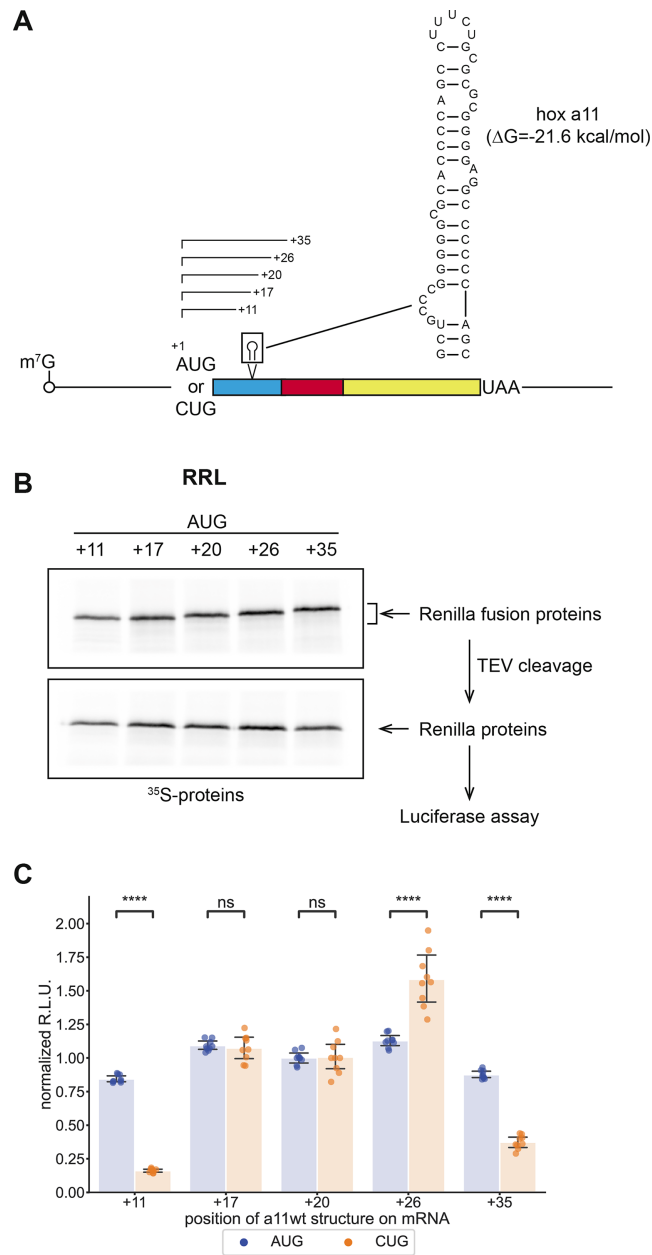
Figure 2. Translation initiation on CUG is sensitive to the position of the downstream secondary structure. (A) Schematic representation of the RNA reporters highlighting the two AUG or CUG initiation codons used and the wild-type a11 hairpin, which is inserted at +11, +17, +20, +26 or +35 positions. (B) Representative SDS-PAGE of in vitro translation products obtained with AUG reporters in RRL. The upper panel shows the 35 S-labelled products before TEV cleavage, the lower panel shows the 35 S-labelled products after TEV cleavage. Proteins produced by TEV cleavage were used for Luciferase assays. (C) Quantification of Renilla luciferase luminescence produced in RRL from a11-RNA reporters initiating with an AUG codon (blue) or with a CUG codon (orange). Relative luminescence units (R.L.U.) were normalized to those obtained with the +20 AUG reporter for all AUG reporters or with the +20 CUG reporter for all CUG reporters. Bar heights show mean normalized ratios and error bars represent the corresponding 99% confidence interval using the t -distribution. P -values were calculated using a Student t -test for independent samples. *: 0.01 < P < 0.05, **: 0.001 < P < 0.01, ***: 0.0001 < P < 0.001, ****: P < 0.0001
